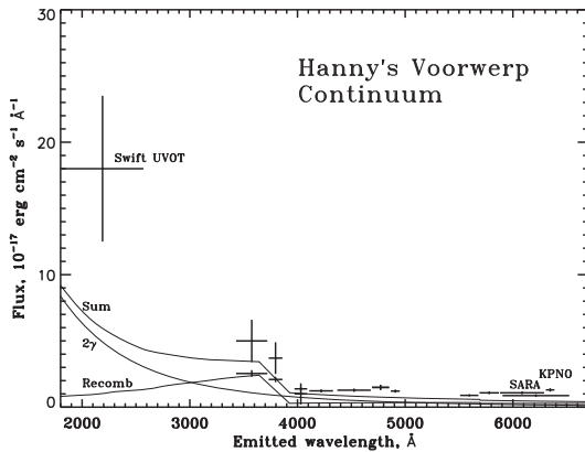
Figure 8. The continuum from Hanny's Voorwerp. Binned regions of the spectra from strong emission lines are combined with imaging results. The error bars on the UV point from Swift reflect maximum and minimum corrections for [C III] \lambda 1909 emission. The curves show the contribution of nebular continuum emission ('Recomb'), two-photon emission ('2 \gamma '), an empirical approximation for the pseudo-continuum of blended high-order Balmer emission lines between 3646 and 3950 Å and the sum of all these components. Scaled to match the observed equivalent width of H \beta , these sources dominate the blue peak in the continuum, but fall short by about a factor of 4 in the red and likewise leave much of the UV continuum unaccounted for. These regions may thus include contributions from imbedded starlight or dust scattering of radiation from the ionizing source.
