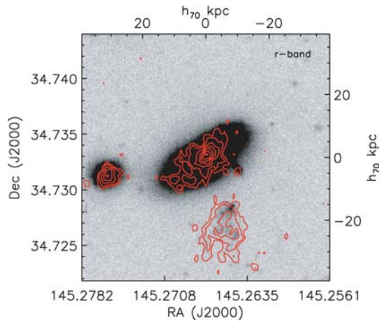
Figure 5. Image of the field obtained after 4700-s exposure with the UV/optical telescope on Swift . The UV data are shown as contours overlaid on a r -band image from SDSS. Both IC 2497 (the central source) and the Voorwerp are strong UV sources.
