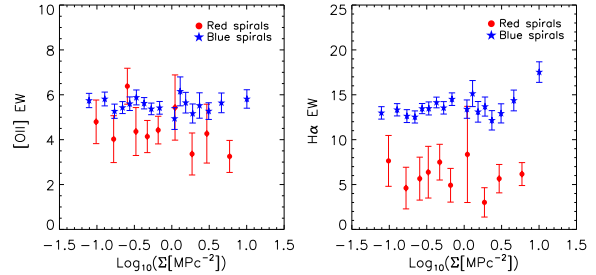
Figure 10. The median equivalent widths of [OII] and \text{H}\alpha as a function of local galaxy density. Blue and red spirals are shown as blue stars/red dots respectively. Error bars show our estimate of the 1\sigma error on the median value.
