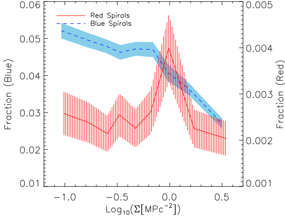
Figure 8. Fraction of red spiral galaxies (red solid line) and blue spirals (blue dashed line) relative to all types of SDSS galaxies in our volume limited sample plotted versus environment as measured by \Sigma . The error regions are also shown; note that the binning is the same for both red and blue spiral samples, and adjusted to have \sim 30 red spirals per bin.
