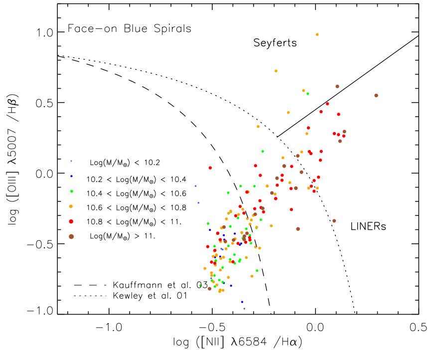
Figure 13. Distribution on the BPT diagram of our sample of face-on disk blue spiral galaxies with the same number of objects in each mass bin as the red spirals shown in Figure 12 (selected randomly). The size and colour of the points indicates the stellar mass of the galaxies (as labelled).
