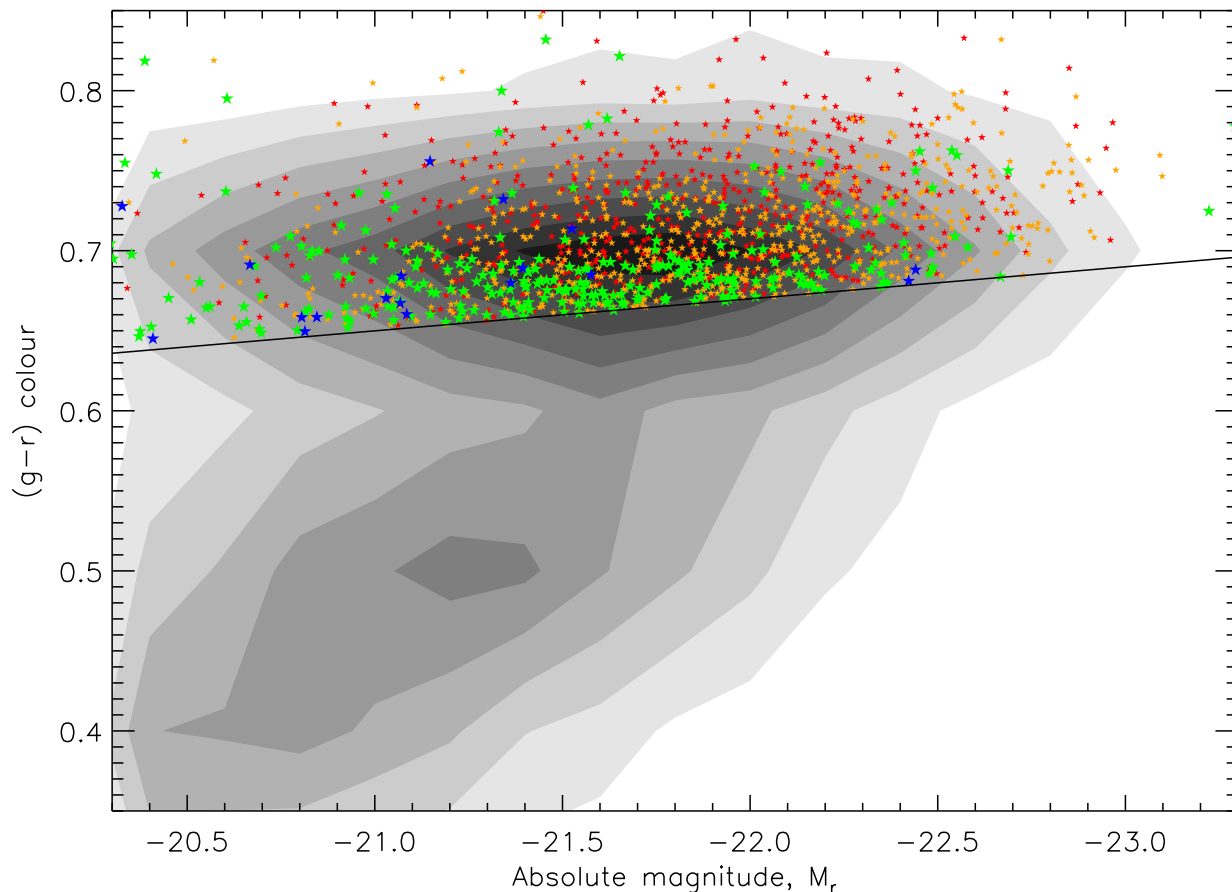
Figure 1. Colour magnitude diagram of the “face-on” ( \log(a/b) < 0.2 ) volume limited clean GZ1 sample. The greyscale contours show the location of galaxies in the red sequence and blue cloud. The solid line indicates the blue edge of the red sequence of GZ1 early types. All red spirals (having visible spiral arms) are shown colour coded by f_{DeV} (blue: f_{DeV} < 0.1 , which roughly corresponds to type Sd; green: 0.1 < f_{DeV} < 0.5 , or Sb-Sc; orange: 0.5 < f_{DeV} < 0.9 , or Sa-S0/a; red: f_{DeV} > 0.9 which are spirals having very large bulges - but note that spiral arms are still visible here, so these are not S0s.). Our final red spiral sample selects only those galaxies with f_{DeV} < 0.5 ( i.e. the blue and green points) to select against spirals dominated by light from the bulge.
