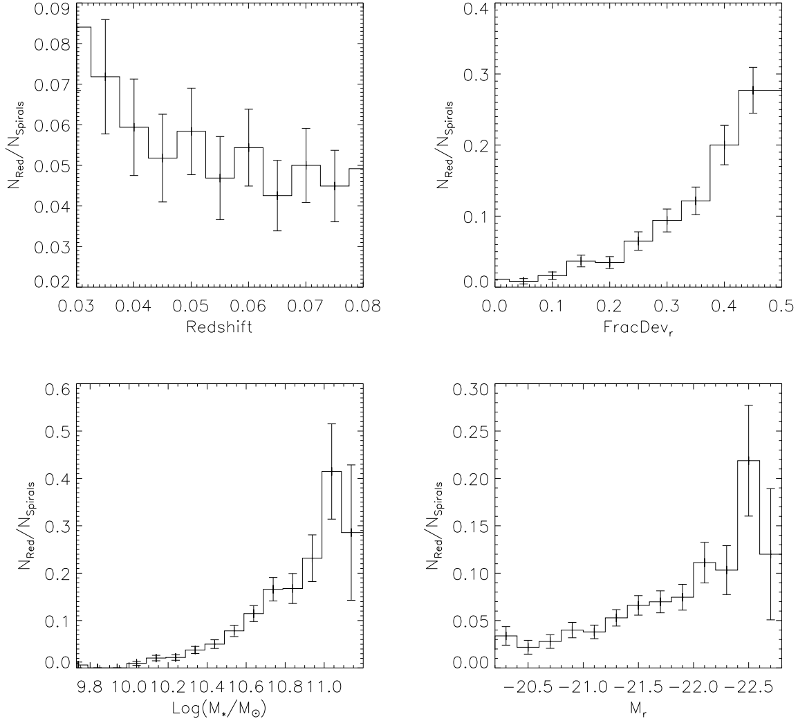
Figure 2. This figure shows the fraction of all face-on, disk-like GZ1 spirals which are found to be red ( i.e. N_{\text{Red}}/N_{\text{Spiral}} ) as a function of (1) redshift, (2) fracdev (or bulge size), (3) stellar mass, and (4) r -band absolute magnitude. \sqrt{N} counting errors are shown.
