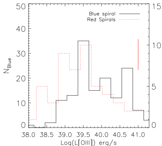
Figure 15. Histogram of [OIII] luminosities of optically identified Seyferts and LINERS in the red spirals (red dotted line) and blue spirals from the mass matched sample (black solid line). The typical error on the red spiral histogram is indicated, offset for illustration purposes. Note that the y -axes are scaled such that the total area under each histogram is equal.
