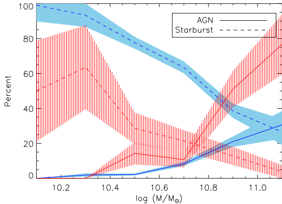
Figure 14. Fraction of galaxies in a given stellar mass range which are classified as "AGN" (Seyfert+LINER) or starforming from the BPT diagram (expressed as a percentage; note that the fraction classified as composites are not shown). The trends for blue spirals are shown with the blue lines, red spirals by the red lines. Shaded regions show the \sqrt{N} counting errors on the fractions. Obviously these errors break down where the fractions approach zero or one, but give a reasonable estimate elsewhere.
