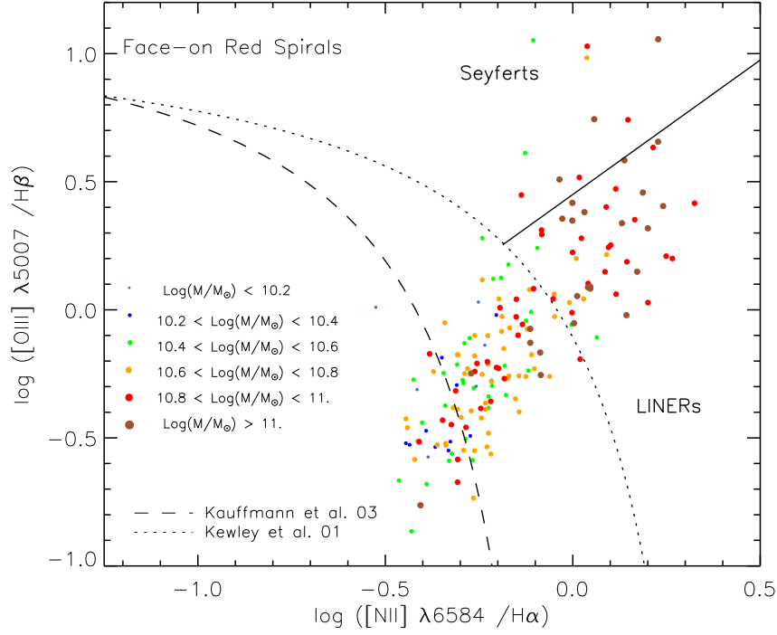
Figure 12. Distribution of face-on disk red spiral galaxies in BPT diagram. The size and colour of the points indicates the stellar mass of the galaxies (as labelled). The diagonal dividing line for LINERs/Seyferts is taken from Schawinski et al. (2007).
