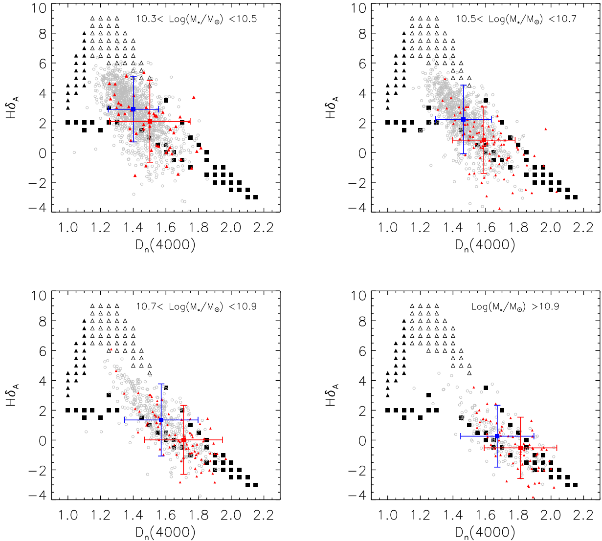
Figure 7. H\delta_A versus D_n(4000) is plotted for our sample of blue and red face-on, disk spirals. In each panel the blue spirals are shown by grey circles, and the red spirals are shown by red triangles. The red and blue error bars indicate the interquartile ranges for the red and blue spirals respectively. The different panels show the evolution with stellar mass, with the lowest mass galaxies at the upper left, down to the highest masses at the lower right. The red spiral galaxies on average show older stellar populations and less recent bursts of star formation in every mass bin. The data are plotted over galaxy models of Kauffmann et al. (2003a) showing regions covered by their starbursting (filled triangle), post starburst (open triangle) and quiescent (filled squares) galaxies.
