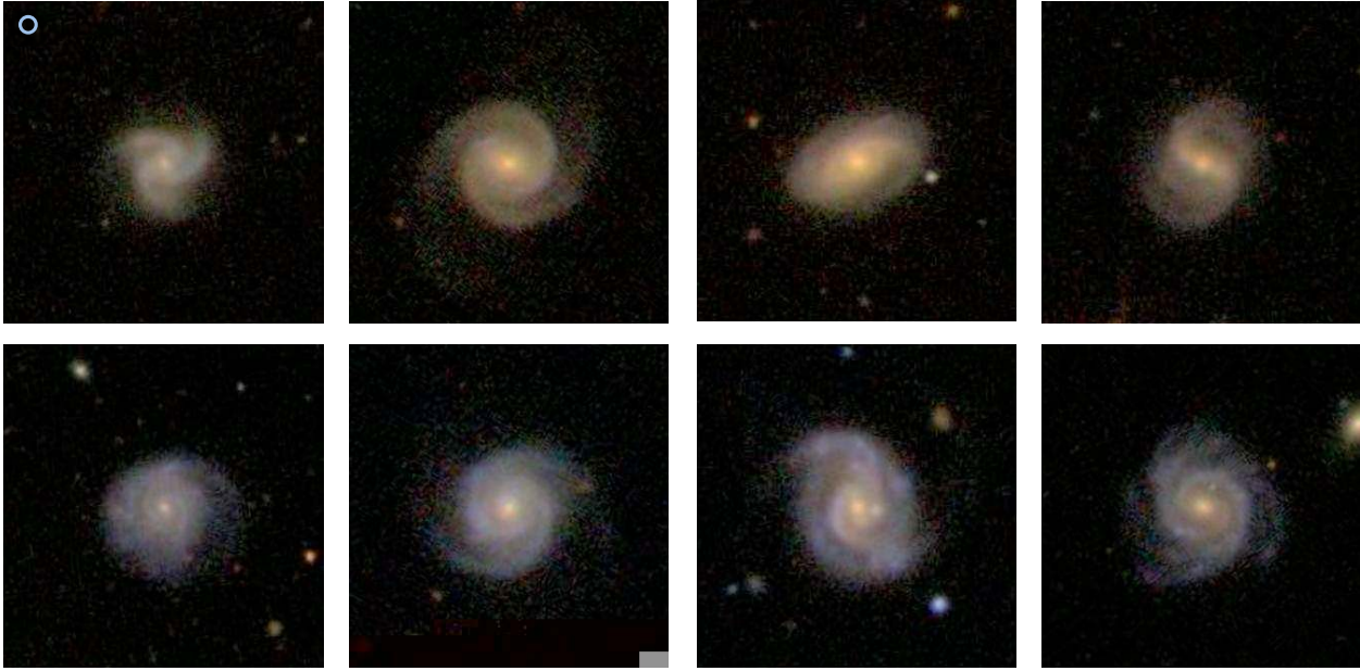
Figure 3. Top row: examples of face-on, red, disk-like spirals with visible arms (as described in the text), Bottom row: face-on, blue, disk-like spirals picked to have similar redshifts, absolute r -band magnitudes, angular sizes and \text{fracdeV} values as the red spiral immediately above them. Images are SDSS gri composites, all 1' \times 1' in size (these are some of the largest angular size galaxies in our sample). The size of the SDSS fibre is indicated at top left of the top left image. Galaxies are (in red/blue pairs from left to right): SDSS J131428.83+334109.2 and SDSS J130058.63+395132.1 at z \sim 0.04 , M_r \sim -20.3 ; SDSS J082959.05+304340.1 and SDSS J100515.00+513545.9 at z \sim 0.05 and M_r \sim -21.7 ; SDSS J104034.48+004902.6 and SDSS J123317.60+575620.1 at z \sim 0.07 and M_r \sim -22.6 ; and SDSS J134248.47+145553.5 and SDSS J155357.57+383923.9 at z \sim 0.08 and M_r \sim -22.3 .
