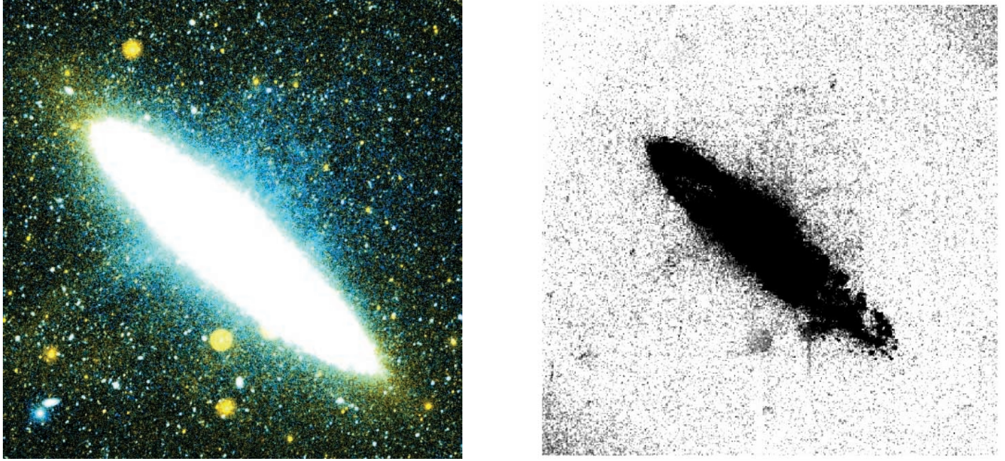
FIG. 1.—NGC 253 in UV and H\alpha . Left : Two-color image, with GALEX NUV in red and FUV in blue. Right : Continuum-subtracted H\alpha image. The images are 30' ( 22.7 kpc) on each side, with north up and east on the left, and are aligned with each other. The intensity scales in both panels are logarithmically scaled and stretched to emphasize the faint, diffuse emission, so the bright disk of the galaxy is saturated.
