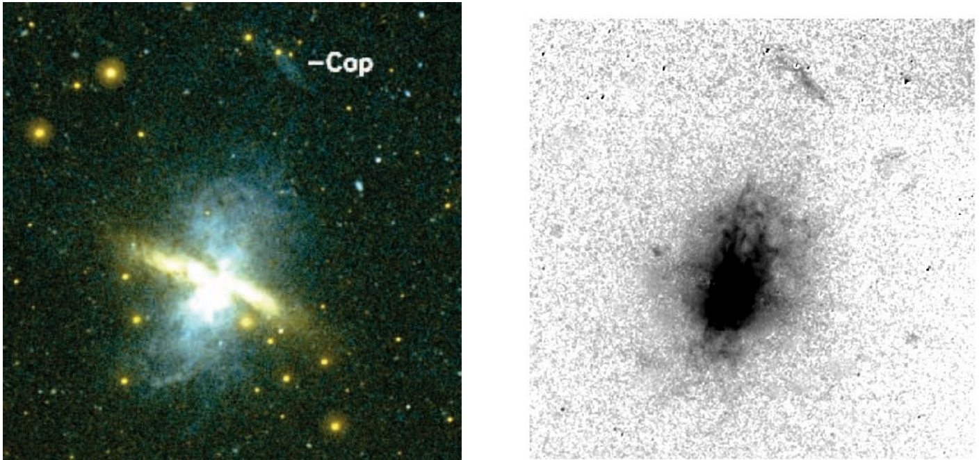
FIG. 2.—M82 in UV and H\alpha . Left : Two-color image, with GALEX NUV in red and FUV in blue. Right : Continuum-subtracted H\alpha image. The images are 21' ( 22.0 kpc) on each side, with north up and east on the left, and are aligned with each other. The intensity scales in both panels are logarithmically scaled and stretched to emphasize the faint, diffuse emission, so the bright disk of the galaxy is saturated.
