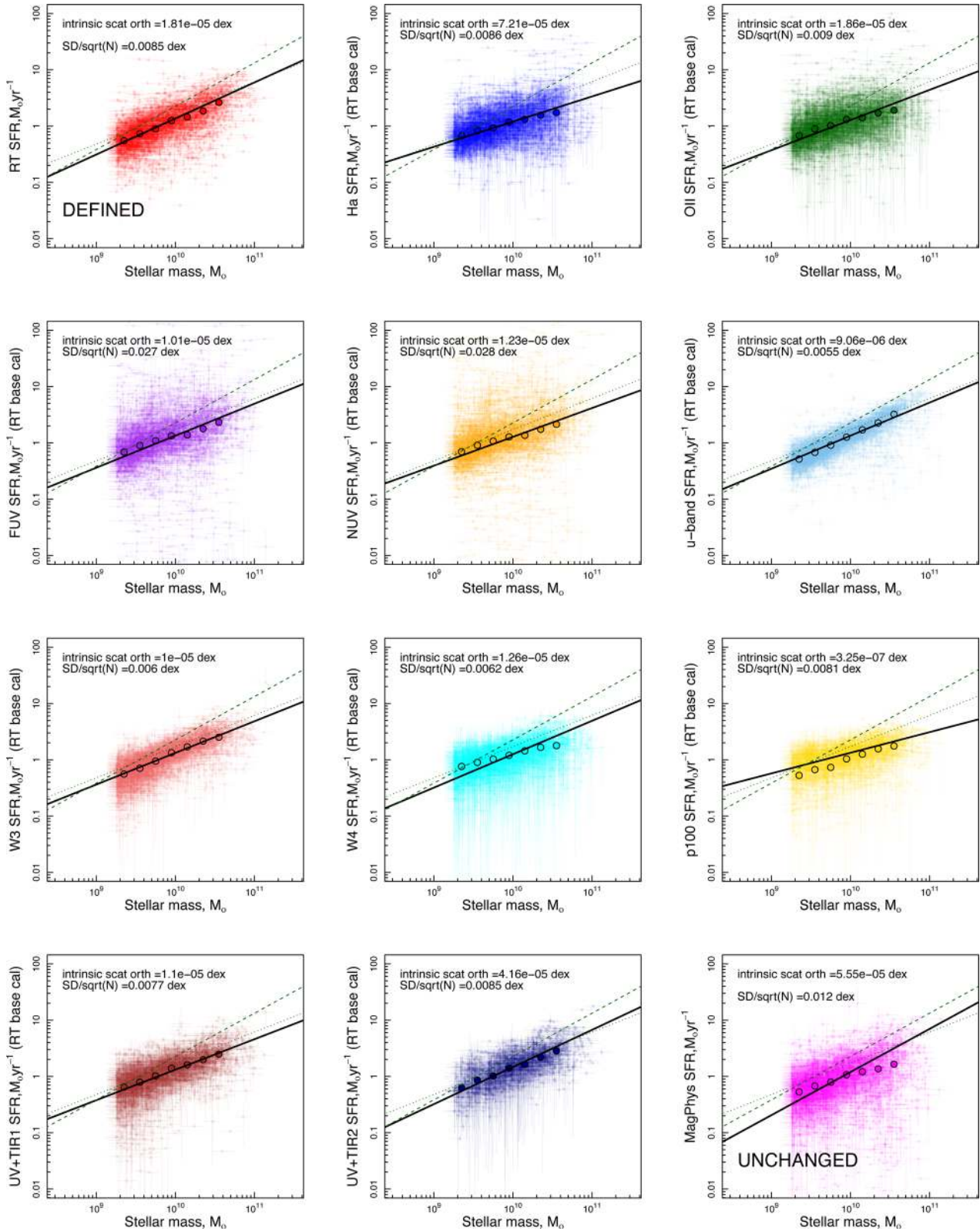
Figure 8. The new SFR– M_* relation derived by calibrating all SFR indicators using the base RT SFR. This figure takes all of the red lines in Fig. 7 (same as the black lines in Fig. 6), calculates an SFR for each observable luminosity in our sample using these calibrations and reproduces the SFR– M_* relation. All orthogonal scatters are improved over the original SFR– M_* relations shown in Fig. 4. The green dashed and dotted show the SFR– M_* relation fits from SDSS at z = 0 (Elbaz et al. 2007) and GAMA I + SDSS at z < 0.1 (Lara-López et al. 2013), respectively. Once again, the large circular points in each panel display the running median of the distribution in log–log space.
