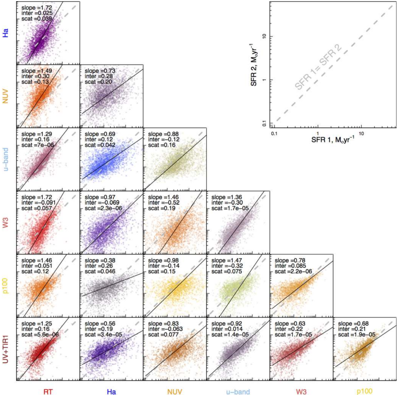
Figure 2. A comparison of selected SFR indicators for the literature SFR calibrations described in Section 3. Both axes display SFR from 0.1 to 50 M_{\odot} \text{yr}^{-1} in log-log space and the grey central dashed line displays a 1:1 relation – shown in the offset panel. In each panel, we display the slope, intercept and orthogonal intrinsic scatter (note that this is the scatter not accounted for by error in the measurement – i.e. a very small scatter implies that the intrinsic scatter in the distribution is much smaller than the measurement error) of the best linear fit. Throughout this paper, we assign a specific colour to each SFR indicator (shown in the axis labels). The colours in this figure represent a combination of the colours assigned to the indicators compared in each panel. Note that the statistical comparison was done on the full optically defined sample selected as defined in Section 2. However, not all points can be displayed due to negative flux measurement in the plotted SFR indicator (see the text for details).
