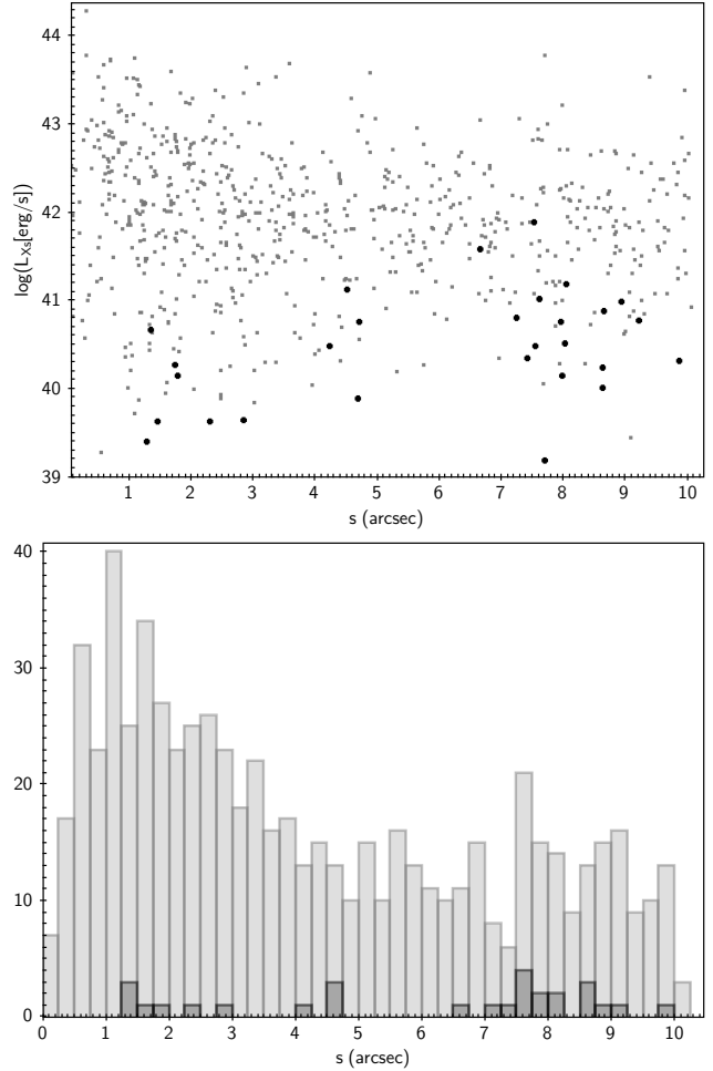
Figure 7. Distribution of angular separations s (in arcsec) between the GAMA (SDSS) and XXL positions for the soft X-ray selected sample. As in the previous figures, sources in low mass galaxies are the filled circles. The bottom panel shows the histogram of the separations for the whole sample (grey) and the low mass sample (black).
