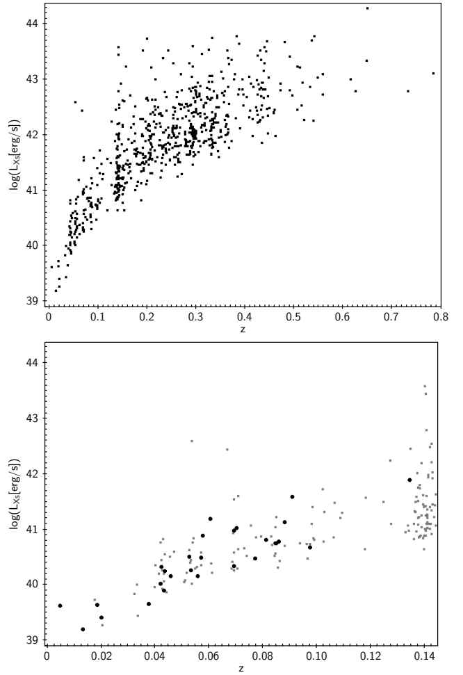
Figure 2. Plot of soft-band X-ray luminosity L_{X_s} against redshift z for the same objects as in Figure 1. Lower panel: Expanded version showing only the galaxies at redshifts out to z=0.145 , approximately the limit for our low mass sample. The latter are shown as filled circles.
