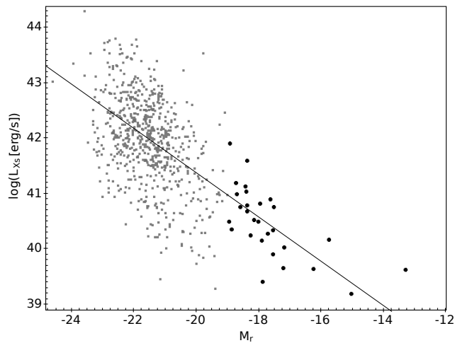
Figure 3. Plot of soft-band X-ray luminosity L_{X_s} against absolute r -band magnitude M_r for the same objects as in Figure 2. Low mass galaxies are again the filled circles. The line indicates the approximate locus of AGN with an Eddington ratio of 10^{-2} (see text).
