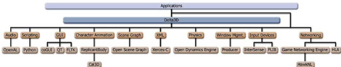
Fig. 1: Delta3D’s architecture, showing the external open source libraries and the type of functionality they provide.
