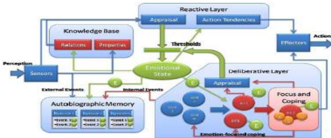
Figure 4: FAtiMA's architecture.
