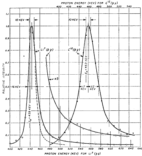
FIG. 2. Thin target excitation curves for the reactions \text{Li}^7(p\gamma) and \text{C}^{12}(p\gamma) . The loss of energy of the incident protons in the targets was approximately 10 kev. The indicated resonance energies at 439 kev and 453 kev were determined from the thick target curves of Fig. 1.
