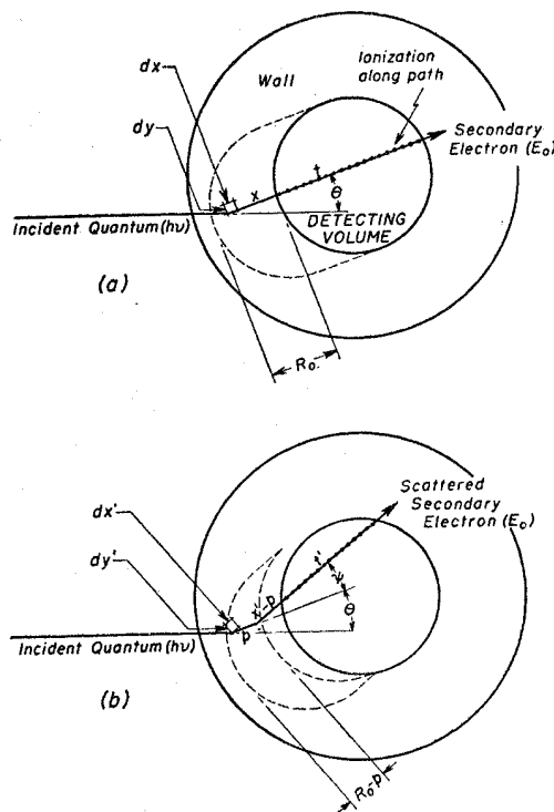
FIG. 12. The detection of secondaries produced by gamma-radiation.
