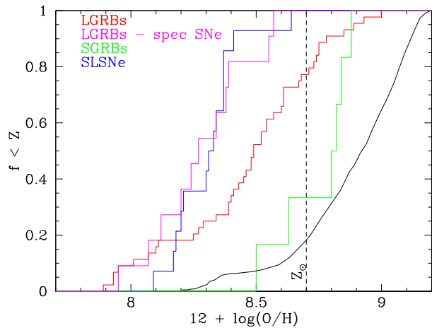
Fig. 3 Host galaxy metallicities for long GRBs from Krühler et al. (2015), short GRBs (from Berger 2009) and SLSNe (from Leloudas et al. 2015). It is striking that the metallicities of LGRBs appear significantly lower than for the SGRBs, or indeed the general galaxy population (Graham and Fruchter 2013). However, those of the GRBs with apparent SNe appear to be somewhat lower still, and are very similar to those observed in SLSNe host galaxies
