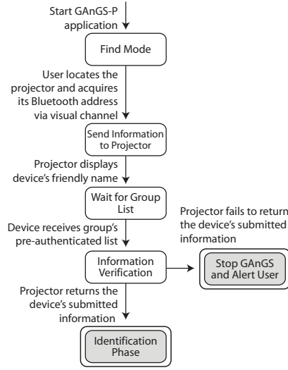
(a) Flow Diagram for a Member Device in GAnGS-P
