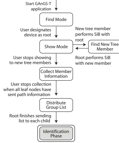
(b) Flow Diagram for the Root Device in GAnGS-T
