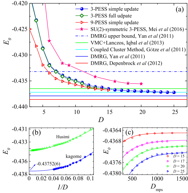
FIG. 1. Ground-state energy of the KHAF. (a) E_0 as a function of D , shown for the 3-PESS and simple-update method up to D = 25 , 3-PESS by full update to D = 13 , and 9-PESS with simple update to D = 15 . Shown for comparison are results from other numerical studies. (b) E_0(D) for the 3-PESS ansatz, shown as a function of 1/D and compared with results obtained for the Husimi lattice [57]. (c) Convergence of E_0(D) as a function of D_{\text{mps}} , shown for several values of D .
