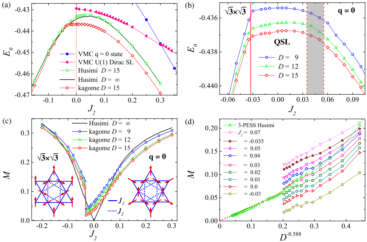
FIG. 3. Energy and staggered magnetization of the KHAF with next-nearest-neighbor coupling. (a) E_0(J_2) calculated with a 9-PESS using D = 15 . Shown for comparison are results for the Husimi lattice with D = 15 and D = \infty , as well as the VMC results of Ref. [14]. (b) Detail of E_0(J_2) near J_2 = 0 ; with increasing D , a cusp-type discontinuity emerges near J_2 = -0.03 (red solid line). The shaded region denotes the location of the continuous transition at small positive J_2 , deduced from the magnetization of panel (d). (c) M(J_2) calculated using D = 9, 12 , and 15 , compared with results for the Husimi lattice at D = \infty . Insets represent the \sqrt{3} \times \sqrt{3} (left) and q = 0 ordered phases (right). (d) M as a function of 1/D^{0.588} , with the Husimi result indicating J_2 values for which M may extrapolate to zero within the error bars.
