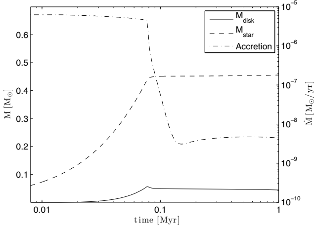
Fig. 4. Evolution of disk mass and stellar mass (solid and dashed line on left scale respectively) and accretion rate onto the star (dash-dotted line on right scale). Adapted from Fig. 5 in Hueso & Guillot (2005).
