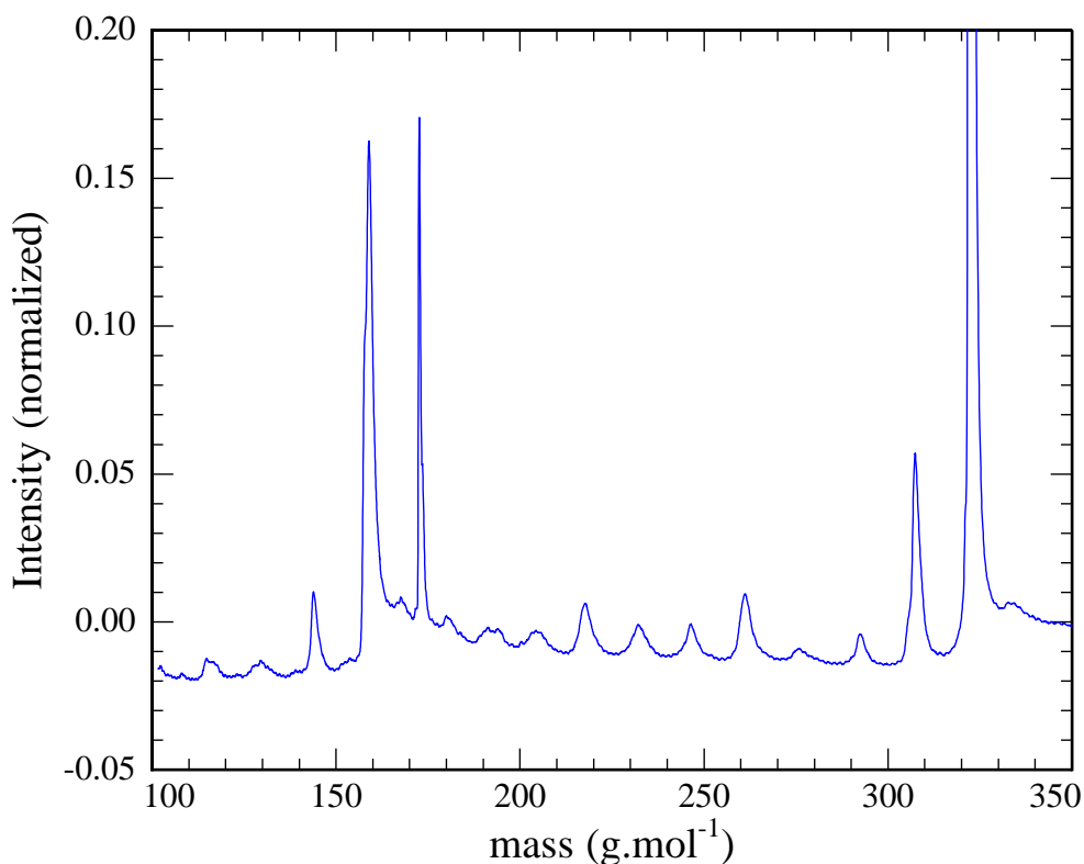
Figure 3: Mass spectrum of molecule 1 for 266 nm pump/800 nm probe summed over -0.5 ps to 1.5 ps, pump/probe delay
