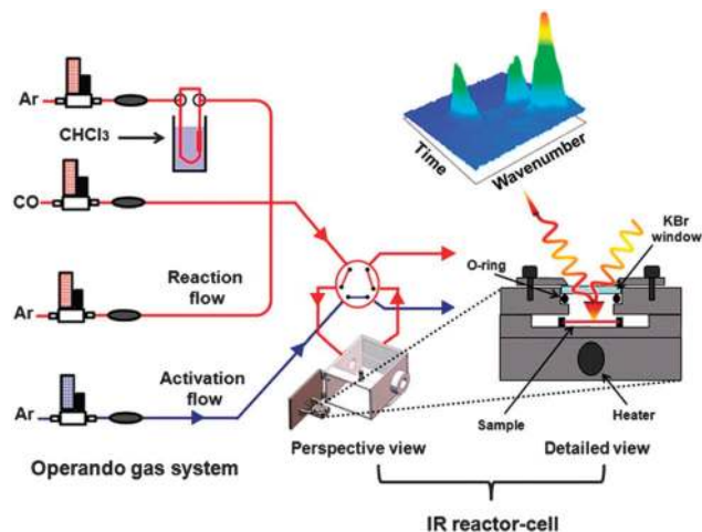
Fig. 14 Schematic of the layout of the in situ IR reactor cell and operando gas detection experimental set-up used by Mintova et al. for detection of carbon monoxide. 159 Reprinted with permission from X. Zou, J.-M. Goupil, S. Thomas, F. Zhang, G. Zhu, V. Valtchev and S. Mintova, J. Phys. Chem. C , 2012, 116 , 16593–16600. Copyright 2012 American Chemical Society.
