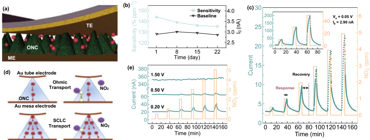
Fig. 8 a Schema of the cross section of the tube/organic/mesa structure. VOPc nanopylramids (green cones) provide sufficient space for NO 2 gas molecules to penetrate the structure. The red particles denote NO 2 gas molecules. b Stability test in ambient atmosphere: sensitivity (left axis) and baseline (right axis) over time. c Response of periodic NO 2 exposure. The device is operated under 0.05 V bias applied to the tube electrode. d Schematic diagram of charge transport and response to NO 2 under ohmic transport (upper panel) and SCLC transport (lower panel) conditions. e Response of organic nanocrystal diode sensor (device 1) at 0.20, 0.50, and 1.50 V bias applied to the tube electrode. Reproduced with permission [65]. Copyright 2018, Wiley–VCH. (Color figure online)
