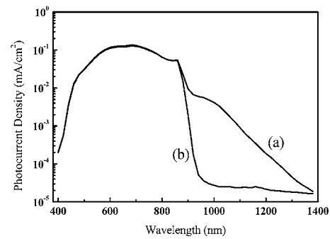
FIG. 3. Spectral response of cells with (line a) and without (line b) GaSb/GaAs type II QDs.
