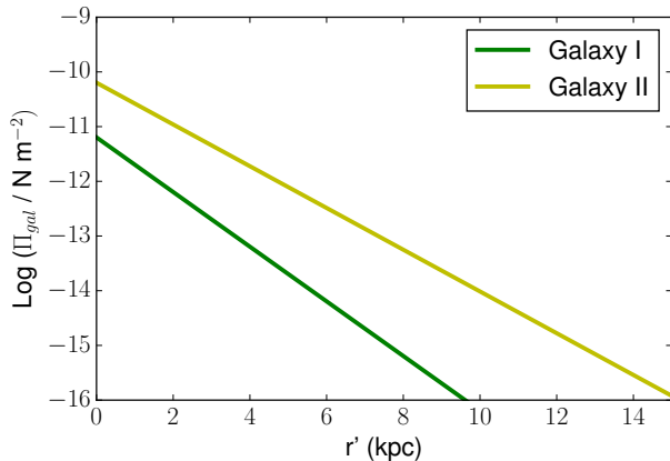
Figure 4. The anchoring force as a function of radial distance from the galaxy centre for two model galaxies (I and II, as indicated).
