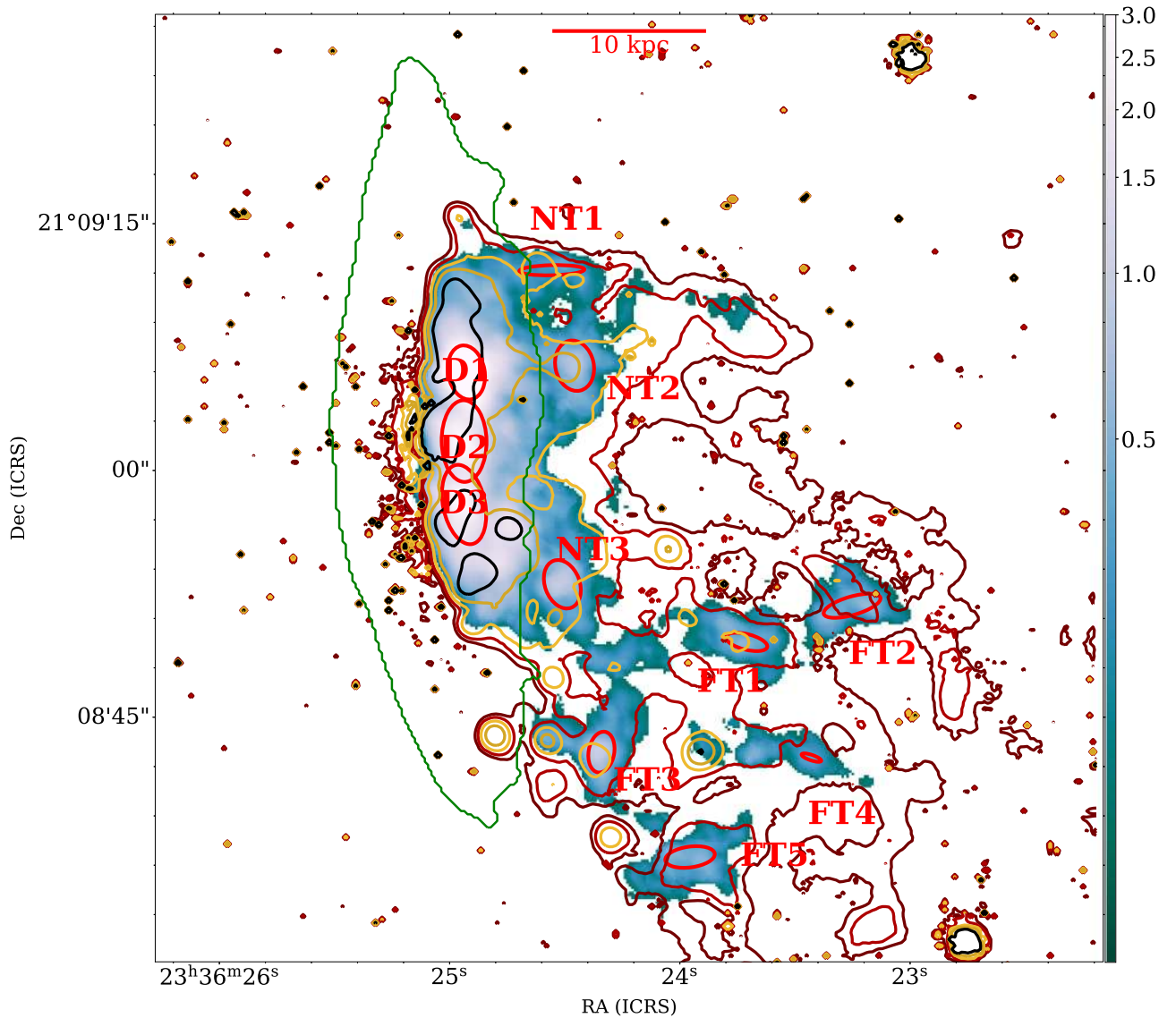
Figure 2. CO(2–1) emission (in Jy/beam km s −1 ) map of JW100 with superimposed the H \alpha contours from MUSE (in different colors, at 2 \times 10^{-17} , 4 \times 10^{-17} , 8 \times 10^{-17} , 1.6 \times 10^{-16} , and 3.2 \times 10^{-15} erg cm −2 s −1 arcsec −2 ) and the regions analyzed in this paper in red (labels D1 to D3 for the disk regions, NT1 to NT3 for the clumps close to the disk, and FT1 to FT5 for the clumps in the far tail). The green contour shows the extent of the stellar disk.
