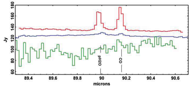
FIG. 3.—Same as Fig. 2, for regions around 79 and 90 \mu\text{m} . The spectra of T Tau and AA Tau have been multiplied by 2 and 150. The emission close to 90 \mu\text{m} is a blend of \text{H}_2\text{O} and \text{CH}^+ , and in HD 100546 is thought to be mostly from \text{CH}^+ .
