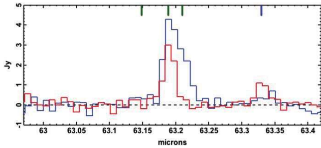
FIG. 7.—Spectrum of [OI]63 \mu\text{m} and \text{H}_2\text{O} from the jet source RW Aur (blue histogram), compared with AA Tau (red histogram), scaled up by a factor of 3 for easier comparison). These spectra are continuum-subtracted, and only the central spaxel is shown. AA Tau is unresolved whereas RW Aur has a prominent redshifted wing in [OI]. The velocities of the three components which dominate the [OI]6300 \text{\AA} line are shown by the green tick marks, at the stellar velocity (heliocentric velocity +23 \text{km s}^{-1} ) and at -190 and +100 \text{km s}^{-1} (Hartigan et al. 1995). Also shown is the wavelength of the \text{H}_2\text{O} line, at the stellar velocity.
