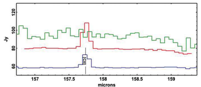
FIG. 4.—Same as Fig. 2 for regions around 145 and 158 \mu\text{m} . The spectra of T Tau and AA Tau have been multiplied by 2 and 150.
