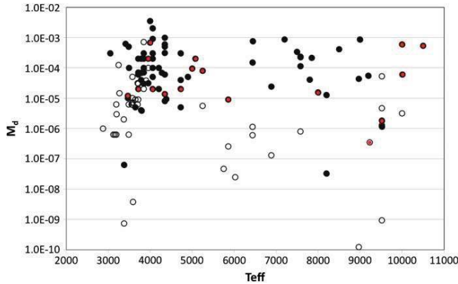
FIG. 10.—Disk dust mass of the GASPS sample, normalised to a distance of 140 pc ( units of M_{\odot} ), plotted as a function of the stellar effective temperature ( in K ). This illustrates the line detectability of a disk of a given dust mass at the distance of the Taurus star forming region. [OI]63 \mu\text{m} detections are shown as filled circles , and open circles depict [OI] upper limits. An additional red dot indicates systems which were detected in [CII].
