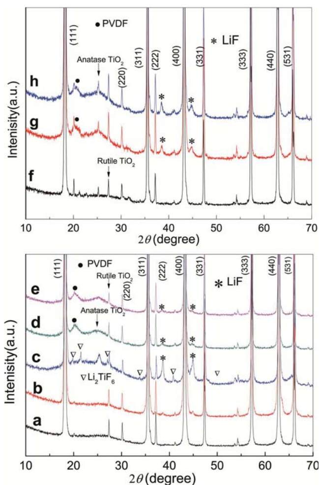
Figure 5 | XRD patterns of LTO and LTO/C. (a) As-prepared LTO. (b) LTO after soaking under Condition A (DEC at 50°C). (c) LTO after soaking under Condition B (1 M LiPF 6 /EC+DMC+EMC at 50°C). (d) LTO in fully charged NCM/LTO battery stored under Condition D. (e) LTO in NCM/LTO battery cycled under Condition E. (f) As-prepared LTO/C. (g) LTO/C in fully charged NCM/(LTO/C) battery stored under Condition D. (h) LTO/C in NCM/(LTO/C) battery cycled under Condition E. Note that the NCM/LTO and NCM/(LTO/C) batteries tested under Conditions D and E were fully discharged before the XRD analysis.
