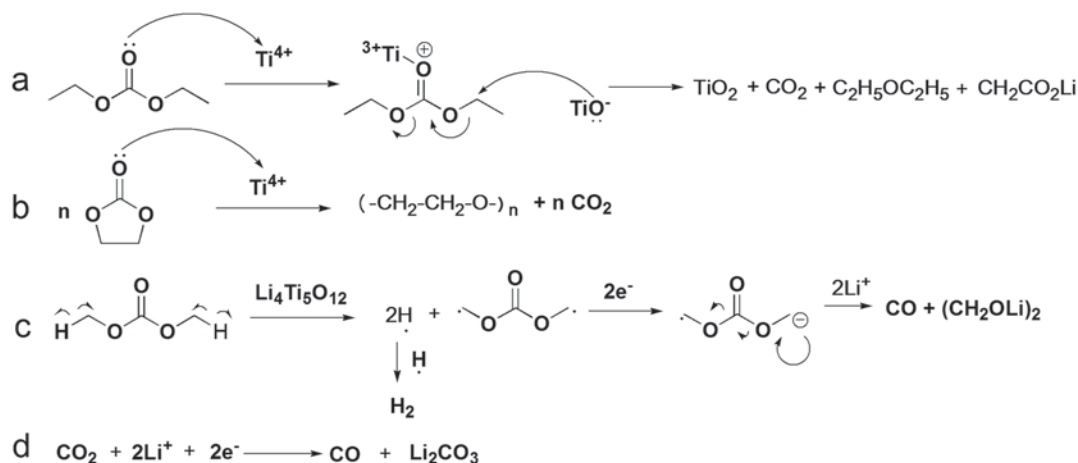
Figure 4 | Tentative gas generation reactions in the gassing of LTO electrode.
