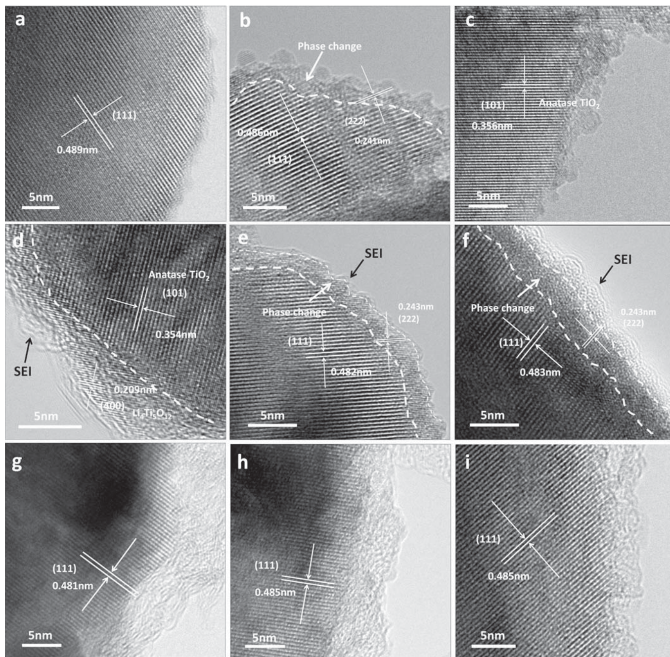
Figure 3 | TEM images of LTO and LTO/C electrodes. (a) As-prepared LTO. (b, c) LTO soaked under Condition A (DEC at 50°C). (d) LTO soaked under Condition B (1 M LiPF 6 /EC+DMC+EMC at 50°C). (e) LTO in fully charged NCM/LTO battery stored under Condition D. (f) LTO in NCM/LTO battery cycled under Condition E. (g) As-prepared LTO/C. (h) LTO/C in fully charged NCM/(LTO/C) battery stored under Condition D. (i) LTO/C in NCM/(LTO/C) battery cycled under Condition E. Note that the LTO and LTO/C batteries tested under Conditions D and E were fully discharged before TEM examination.
