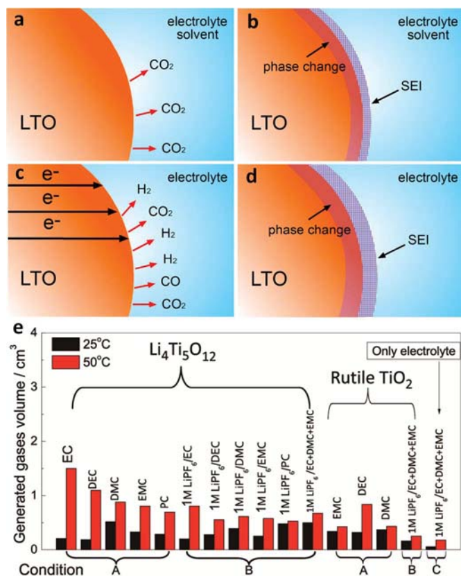
Figure 2 | Schematics of gassing behaviors of LTO electrodes with electrolyte under different conditions. (a) CO 2 is generated when LTO is soaked under Conditions A and B. (b) The surface of LTO is covered by solid electrolyte interface (SEI) film consisting of the reaction products of LTO with solvents or electrolyte solution, and the phase change occurs at the outermost surface of LTO soaked under Conditions A and B. Note that the components of SEI film formed under Conditions A and B is obviously different. (c) Gaseous H 2 , CO 2 and CO are generated when NCM/LTO batteries are stored and cycled under Conditions D and E. (d) The surface of LTO is covered by a SEI film consisting of the reaction products of LTO with electrolyte under Conditions D and E, and phase change occurs at the outermost surface of LTO. Note that the thickness of SEI film under Conditions D and E are obviously different. (e) Volumes of gas generated when LTO or rutile TiO 2 is soaked under Conditions A, B and C.
