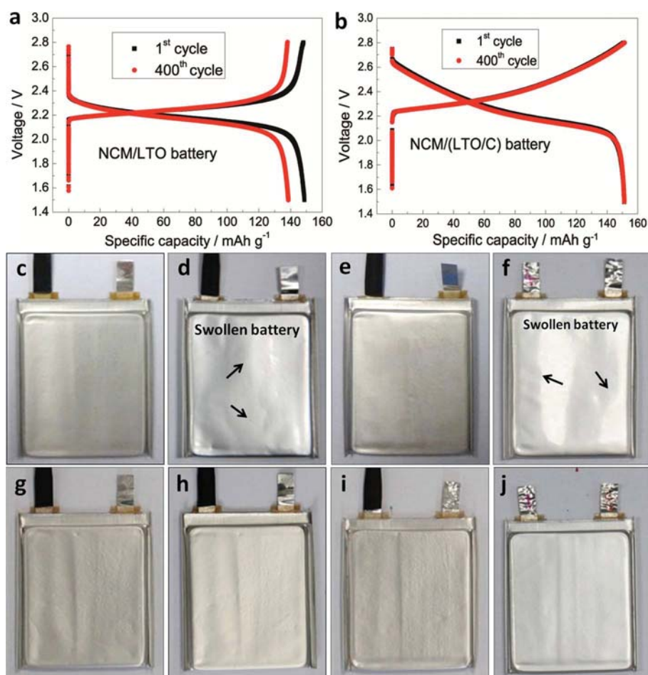
Figure 1 | Cyclic and storage performance of NCM/LTO and NCM/(LTO/C) batteries under Conditions D and E. (a, b) Performance curves at 0.5C/0.5C and 25°C (Condition E). Photographs of soft-packed NCM/LTO batteries (c) before and (d) after storage under Condition D, and (e) before and (f) after cyclic test under Condition E. Photographs of soft-packed NCM/(LTO/C) batteries (g) before and (h) after storage under Condition D, and (i) before and (j) after cyclic test under Condition E. Note that swelling caused by gassing is observed in the NCM/LTO batteries (arrows (↑) labels the obviously swollen areas), but not in the NCM/(LTO/C) batteries.
