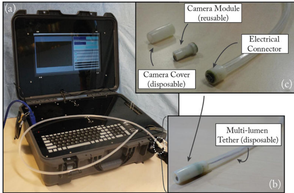
Fig. 2. (a) HydroJet platform designed to be easily transportable. (b) Picture of the HydroJet capsule. (c) The HydroJet capsule disassembled into disposable and reusable components.
