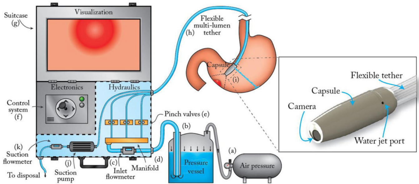
Fig. 1. Diagram of the HydroJet system: (a) Air pressure tank, (b) Dispensing pressure vessel, (c) Inlet flowmeter, (d) Manifold, (e) Pinch valves, (f) Control system, (g) Suitcase, (h) Multi-lumen tether, (i) Capsule, (j) Suction pump, (k) Suction flowmeter.
