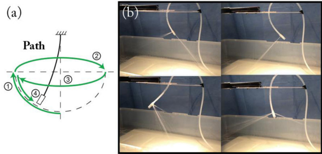
Fig. 7. (a) Programmed path. (b) Pictures of the HydroJet capsule travelling around the programmed path to characterize the full workspace.
