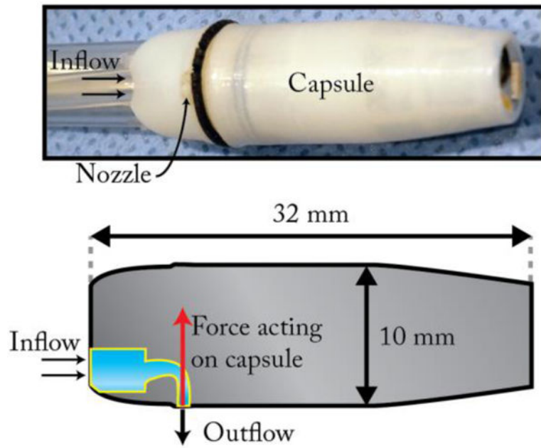
Fig. 3. Capsule cross-section. Three miniature nozzles are carved inside the capsule body with a spacing of 120^\circ around the diameter.
