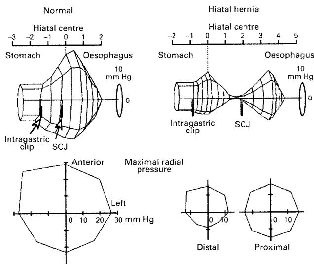
Figure 1. Axial (top) and radial (bottom) pressure topography of the gastroesophageal junction of normal subjects and patients with a hiatus hernia. Position zero on the axial scale is the midpoint of the diaphragmatic hiatus. The proximal clip indicates the median position of the squamocolumnar junction (SCJ) and the distal clip marks the median position of the intragastric aspect of the gastroesophageal junction as imaged endoscopically. With permission (24).
