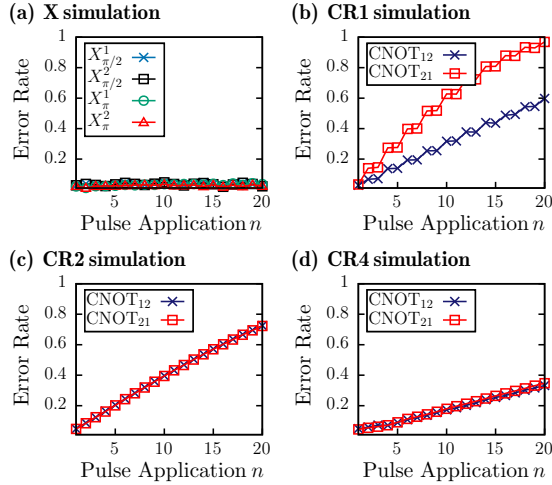
FIG. 2. Evolution of the error rate given by Eq. (13) after n applications of a certain gate. (a) Single-qubit Gaussian derivative pulses defined by Eq. (8); (b)–(d) two-qubit CNOT gates based on the cross-resonance effect. While CR1 includes only one CR pulse on each of the transmons, CR2 and CR4 employ additional X gates to echo out certain errors (see Sec. II and Appendix B).
