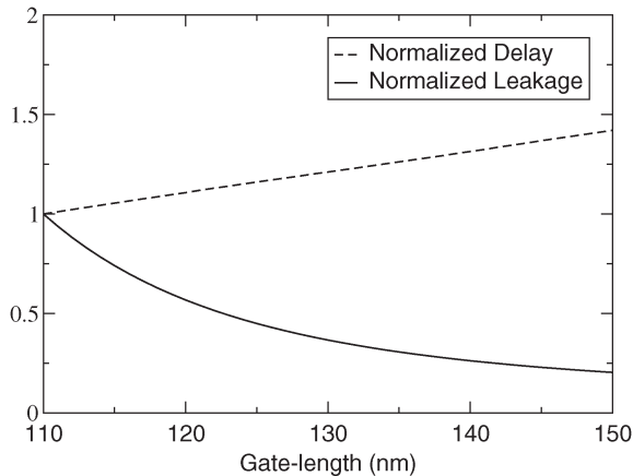
Fig. 1. Variation of leakage and delay (each normalized to 1.00) for an NMOS device in an industrial 130-nm technology.
