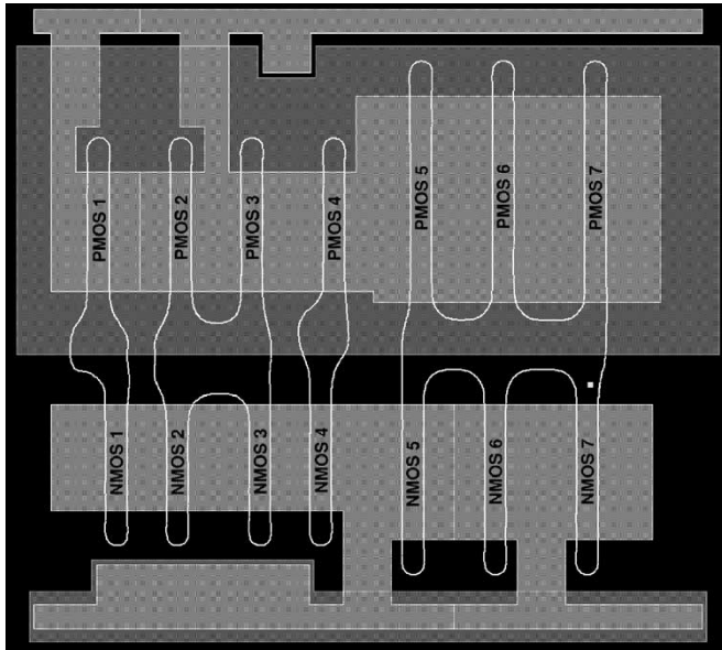
Fig. 4. Cell layout of a generic AND2X6 with simulated printed gate lengths.
