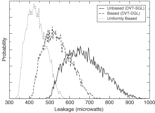
Fig. 5. Leakage distributions for unbiased, uniform-biased, and technology level selectively biased alu128. Note the “left shift” of the distribution with the introduction of biased devices in the design.
