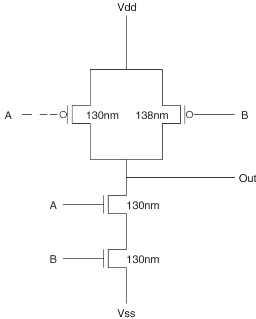
Fig. 3. Gate-length biasing of the transistors in NAND2X1 when only the rise and fall timing arcs from input A to the output are critical.
