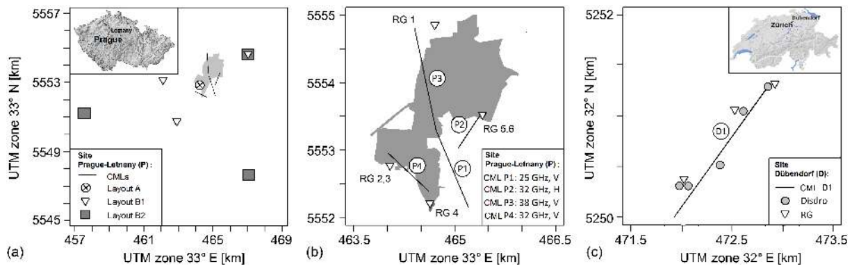
Figure 1. Experimental sites Prague-Letňany, CZ (left and middle panels), and Dübendorf, CH (right panel). Left panel: overview CZ, RG layouts used for CML adjusting. Middle panel: detailed view on CZ, CMLs, and reference RGs. Right panel: detailed view on CH, CML, and the layout of reference disdrometers and RGs.
