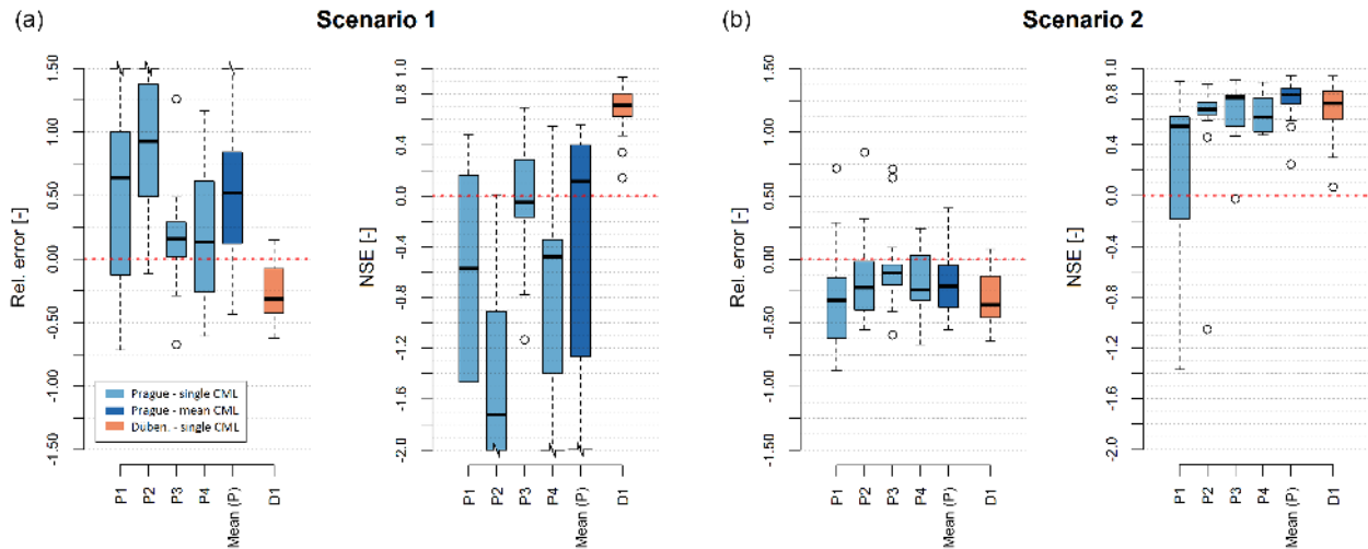
Figure 6. Relative error and NSE in QPEs of unadjusted CMLs evaluated for all events. Each box plot depicts one CML (i.e. CML mean). Scenario 1: QPEs based on models with parameters from the literature. Scenario 2: QPEs based on models with optimal parameters. It can be seen that choosing parameter values for the retrieval model from literature leads to large positive bias (scenario 1, relative error). Conditioning the model on observations leads to a negative bias, albeit with reduced variance. Both do not achieve the virtually unbiased observations obtained with our adjustment method, which are an order of magnitude lower (Fig. 2). The comparably good performance of the CML D1 is due to an exceptional ground truth, which enabled a custom-made wet antenna correction.
