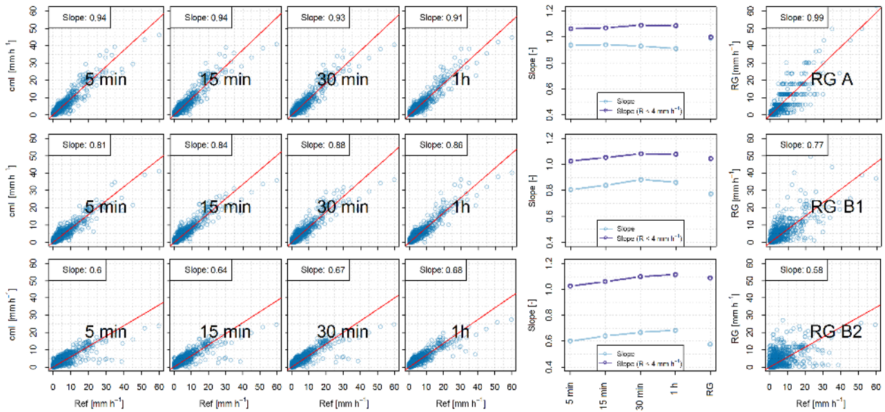
Figure 4. Comparison of mean QPEs from four CMLs to reference rainfall. CMLs are adjusted by rainfall from three different RG layouts (rows) with aggregation intervals of 5, 15, 30 min, and 1 h (four panels on the left), in addition, rainfall from the RG layouts alone is compared to the reference areal rainfall (right panel). Linear trend-line intersects are set to zero. The middle panel plots the relationship between the slope of the trend lines and aggregation times as well as the slope of the RG layouts.
