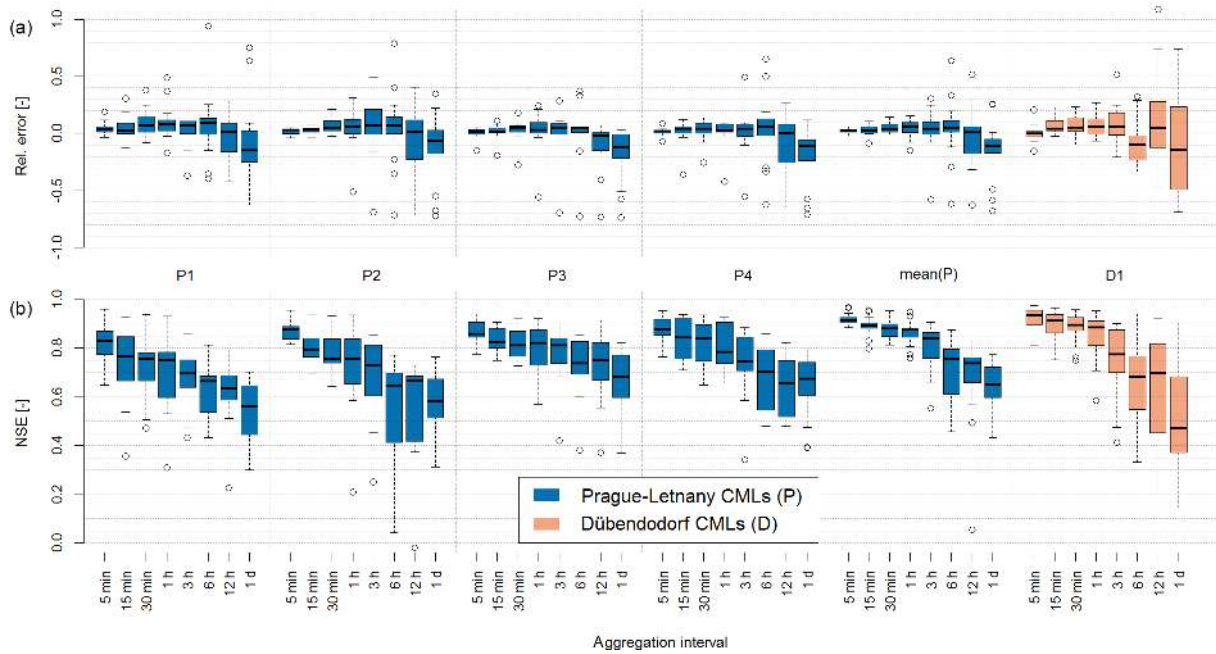
Figure 2. Relative error (top panels) and Nash–Sutcliffe efficiency coefficient (NSE) (bottom panels) in QPEs of CMLs adjusted by rainfall data of different time resolution. Each CML layout is represented by eight box plots corresponding to QPEs adjusted by rainfall aggregated to time intervals from 5 min to 1 day. Each box plot depicts a range of the statistics during all evaluated events. Five groups of blue box plots (left panel) evaluate QPEs from single CMLs and from their average at Prague-Letňany. One group of orange box plots (right panel) depicts QPEs from a single CML at Dübendorf.
