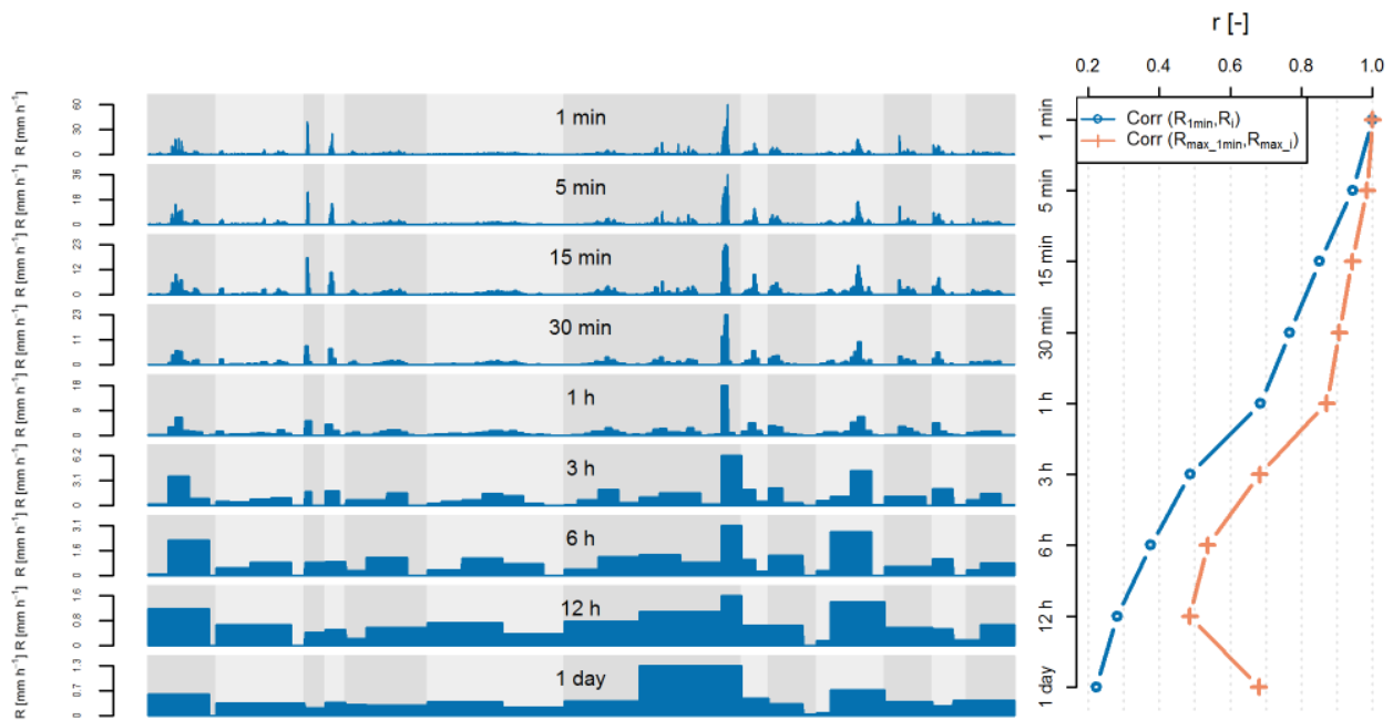
Figure A1. Rainfall peaks smoothed out by longer aggregation intervals, here shown for the case study in Prague-Letňany (CZ). Left panels: merged time series of 13 events aggregated to time steps from 1 min to 1 day. Vertical stripes indicate individual events. Note how the range of the y axis decreases from the top to the bottom row. Right panels: correlation between time series with 1 min resolution and the other time series of different resolutions (blue) and correlation between peak intensities of events derived from rainfall data with 1 min resolution and peak intensities derived from aggregated rainfall data (red).
