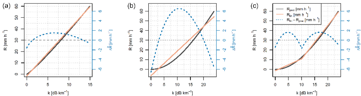
Figure 7. Performance of linear approximation of k – R models for vertically polarized 38 GHz CML in terms of rainfall intensity. Left panel: linear approximation (red) of the power-law model (black). The blue dashed line shows the resulting model structure errors. Middle panel: linear approximation of power-law model coupled with Kharadly's wet antenna attenuation model. Right panel: power-law model combined with Kharadly's wet antenna attenuation model approximated by two linear models fitted separately for light ( R \leq 12 \text{ mm h}^{-1} ) and heavy rainfall events ( R > 12 \text{ mm h}^{-1} ).
