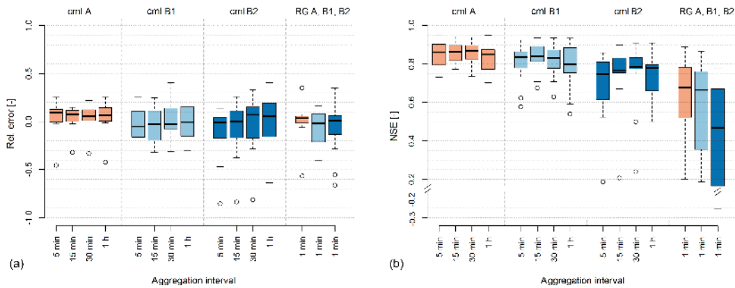
Figure 5. Relative error (left panel) and NSE (right panel) in QPEs from CMLs when adjusted using three different RG layouts (A, B1, B2) and four different aggregation intervals (5, 15, 30 min, and 1 h). Right three box plots in both figures correspond to RG observations of each layout when used alone without CMLs.
