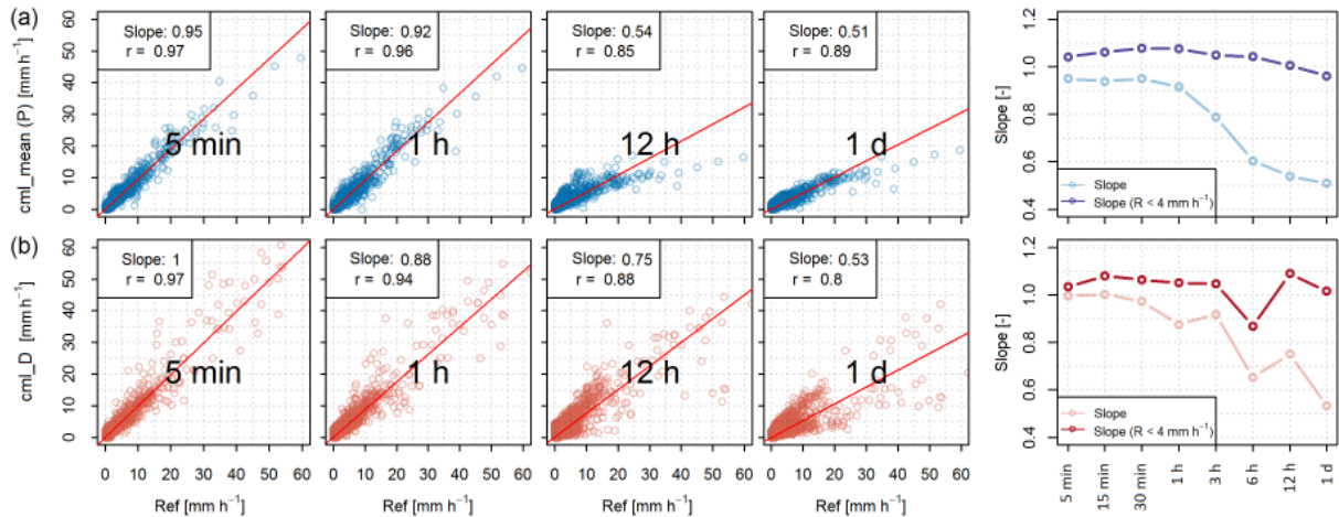
Figure 3. Comparison of CML QPEs adjusted by rainfall data of different time resolution to reference rainfall, from four averaged CMLs in Prague-Letňany (top panels) and one CML in Dübendorf (bottom panels). Scatter plots are shown only for selected aggregation intervals. Linear trend-line intercepts are set to zero. Slopes of trend lines for all aggregation intervals are depicted in the right panels, showing also slopes of trend lines calculated for light rainfalls ( R < 4 \text{ mm h}^{-1} ).
