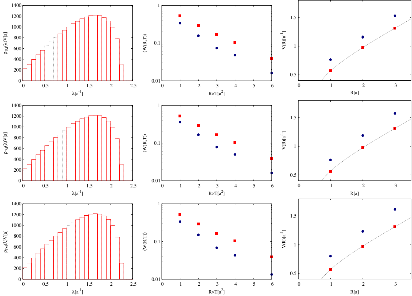
FIG. 8 (color online). The left panels show the intermediate (IM)-cut Dirac spectral density \rho_{\text{IM}}(\lambda) : The IM Dirac modes of 0.5-0.8[a^{-1}] (top panel), 0.8-1.0[a^{-1}] (middle panel), and 1.0-1.2[a^{-1}] (bottom panel) are cut. The central panels show the IM-cut Wilson loop \text{Tr}W^P(R, T) (circles) after removing the IM Dirac modes, plotted against R \times T . For each case, the slope parameter \sigma^P is almost the same as that of the original Wilson loop (squares). The right panels show the corresponding IM-cut interquark potential (circles), which is almost unchanged from the original one (squares), apart from an irrelevant constant.
