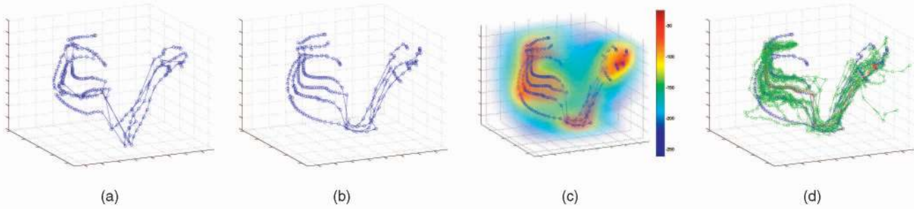
Fig. 4. Models learned from four golf swings from the same golfer. The latent coordinates learned with (a) GPLVM and (b) GPDM are shown in blue. Vectors depict the temporal sequence. (c) -\ln variance for reconstruction shows positions in latent space that are reconstructed with high confidence. (d) Random trajectories drawn from the dynamic predictive distribution using HMC are green, whereas the red trajectory is the mean of the samples.
