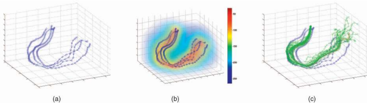
Fig. 9. Models learned with the two-stage MAP from four golf swings from the same golfer. (a) The learned latent coordinates are shown in blue. (b) -\ln variance for reconstruction shows positions in latent space that are reconstructed with high confidence. (c) Random trajectories drawn from the dynamic predictive distribution by using HMC are green, whereas the red trajectory is the mean prediction sample. The distribution is conditioned on starting from the beginning of a golf swing.
