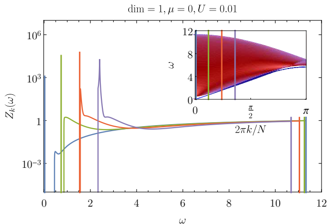
FIG. 7. Peak merging into continuum. We plot the spectral response function Z_k(\omega) relative to a density perturbation for a set of different momenta k . The function is calculated for a set of parameters ( \text{dim} = 1 , U = 0.01 and \mu = 0 ) such that for some values of k the Goldstone mode merges into the continuum spectrum. The plot shows how the delta-like peak of the Goldstone mode transforms into a finite width feature when this merge occurs (purple line).
