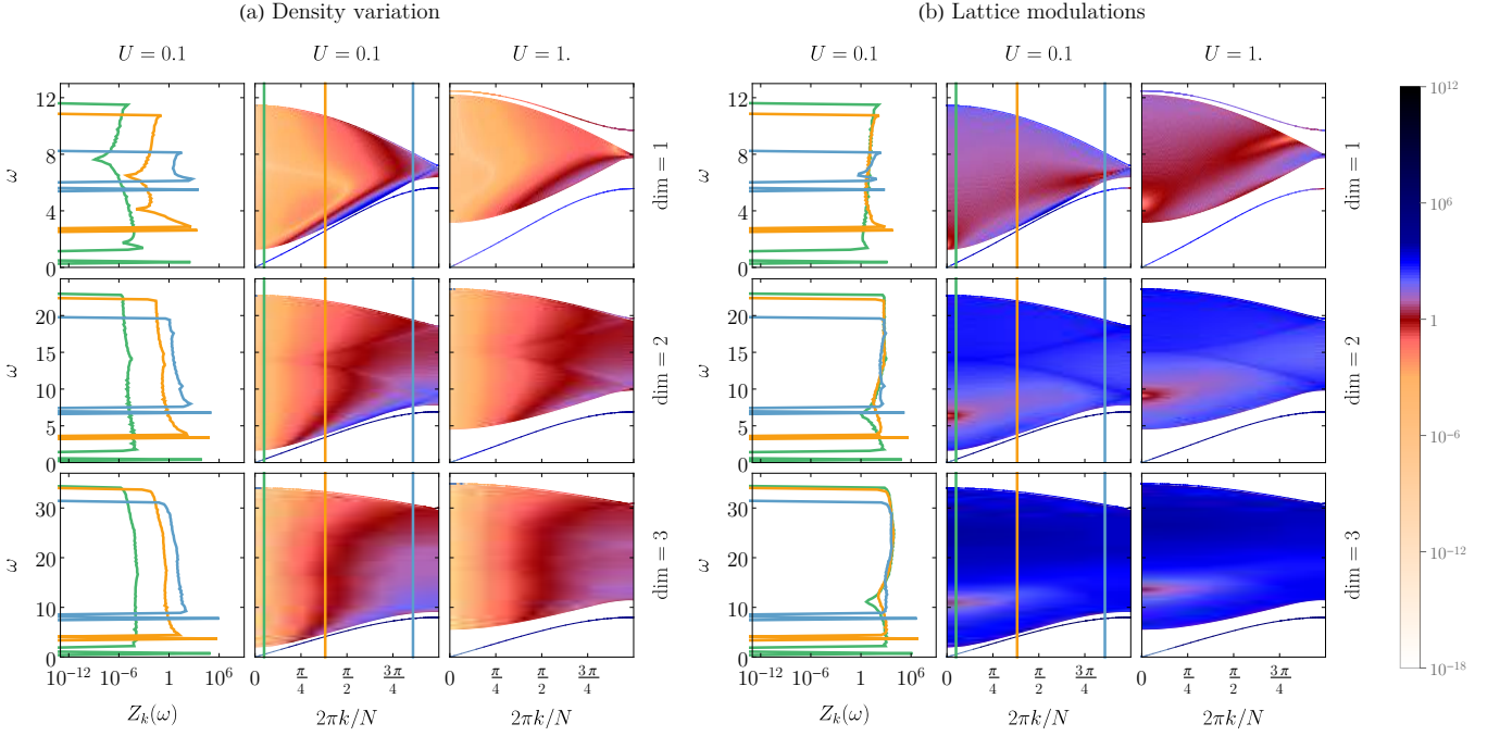
FIG. 5. Spectral functions for (a) Density variation \hat{V}_{\text{density}}^{(k)} from (20) and (b) Lattice modulation \hat{V}_{\text{lattice}}^{(k)} from (21). We show, as colour plots, the values of the spectral response functions Z_k(\omega) in the relevant range of values of k and \omega . In the first column of each panel, we show more logarithmic graphs of Z_k(\omega) for fixed slice of k (indicated by vertical lines of the respective color in the second column). The computations were performed for N = (501, 101^2, 41^3) for \text{dim} = (1, 2, 3) respectively. To extract a continuous response functions, we performed a binning in energy intervals of \Delta\omega = (0.13, 0.2, 0.37) for \text{dim} = (1, 2, 3) respectively.
