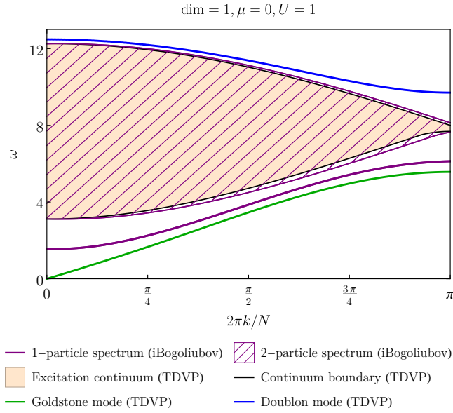
FIG. 11. Comparison of Gaussian TDVP (labelled as TDVP) with iterated Bogoliubov theory. We compare the data of Gaussian TDVP from figure 2 with the 1- and 2-particle spectrum of the non-interacting Hamiltonian of [\hat{H}]_{|\psi_g\rangle} from (C10), which we obtained from the iterated Bogoliubov theory (labelled as iBogoliubov).
