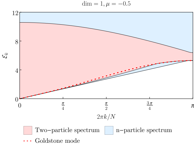
FIG. 9. Bogoliubov spectrum. We show the Bogoliubov dispersion relation \mathcal{E}_k as dashed line (red) within the 2-particle spectrum (light red) which is again embedded into the full excitation spectrum (light blue). Note that \mathcal{E}_k only depends on \mu and the dimension, but is independent of U .
