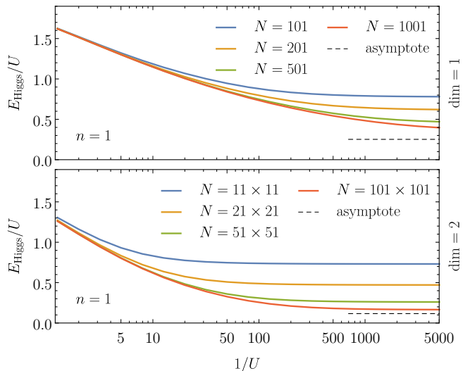
FIG. 4. Continuum/Higgs gap as function of 1/U . This figure shows the gap between the gapless Goldstone mode and the continuum of excitations as a function of 1/U in 1d and 2d and for different system sizes. The asymptotic value for large N and small U obtained in equation (15) is also indicated for N = 1001 in 1d and N = 101^2 in 2d.
