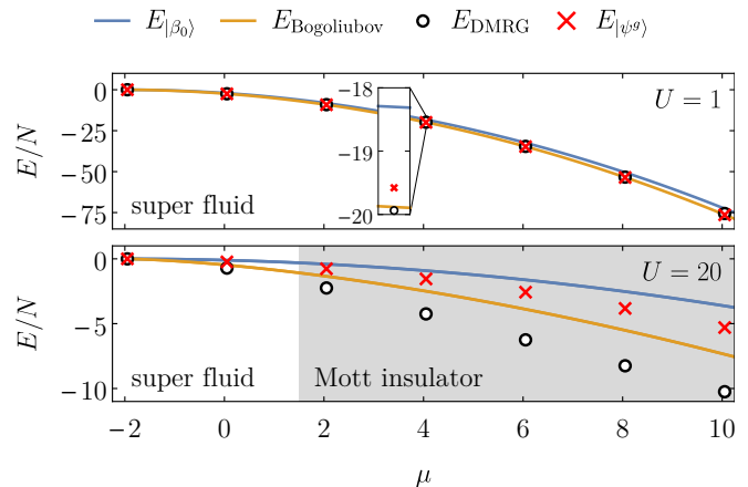
FIG. 1. Comparison of ground state energies in 1d. We compare the following approaches: (a) Minimal energy on manifold of coherent states E_{|\beta_0\rangle} from (A5), (b) Bogoliubov ground state energy E_{\text{Bogoliubov}} = E_{|\beta_0\rangle} - \Delta from (A17) in the limit N \rightarrow \infty , (c) DMRG energy E_{\text{DMRG}} and (d) minimal energy E_{|\psi_g\rangle} of all Gaussian states for N = 501 . The DMRG results were computed for finite systems with open boundary conditions and then extrapolated to the thermodynamic limit N \rightarrow \infty . The Gaussian state energy E_{|\psi_g\rangle} at N = 501 appears to have already substantially reached the thermodynamic limit value.
