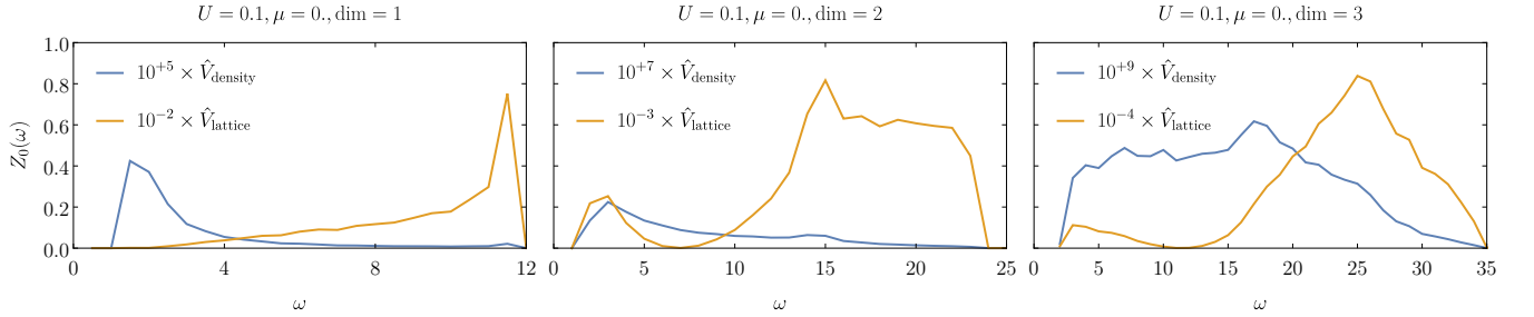
FIG. 6. Comparison: Density variation (20) and lattice modulation (21) at k = 0 . We compare the response functions from density variation with the one from lattice modulations. The response to the lattice modulation is by several orders of magnitude stronger. Note that we rescaled the data by factors of 10^{\pm x} to fit into the same range. The computations were performed for N = (501, 101^2, 41^3) for \text{dim} = (1, 2, 3) respectively. To extract a continuous response functions, we performed a binning in energy intervals of \Delta\omega = (0.5, 1, 1) for \text{dim} = (1, 2, 3) respectively.
