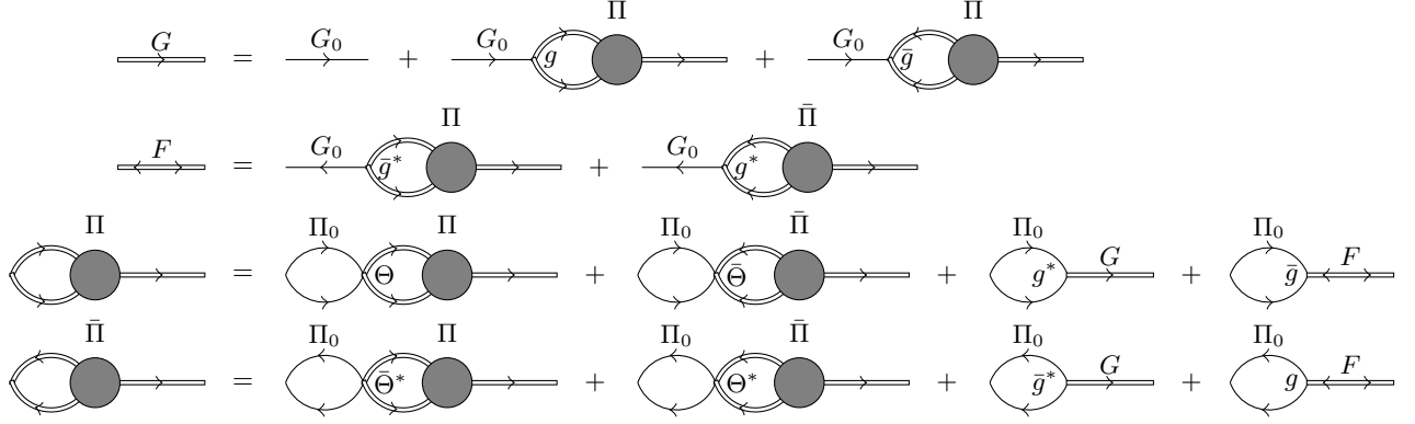
FIG. 12. Feynman diagrams . Pictorial representation in terms of Feynman diagrams of the terms included in equations (G10-G13) for the correlation functions
