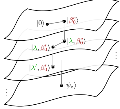
FIG. 10. Iterated Bogoliubov theory. This figure illustrates the procedure of applying the steps of Bogoliubov theory iteratively to find best Gaussian approximation |\psi_g\rangle to the ground state of the Bose-Hubbard model. The individual sheets represent coherent states, i.e. , states with fixed \lambda , but different values of \beta . Traditional Bogoliubov is based on the first two steps from |0\rangle to |\beta_0^c\rangle to |\lambda, \beta_0^c\rangle
