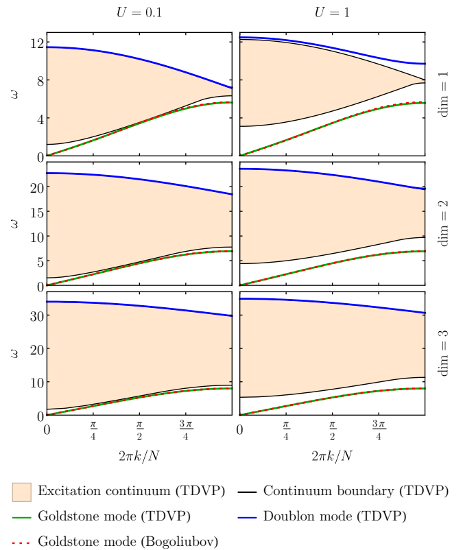
FIG. 2. Excitation spectra for \mu = 0 . We compare the quasi-particle excitation spectrum computed from Gaussian TDVP with Bogoliubov theory. The results are shown for \mu = 0 and two different values of the interaction strength ( U = 0.1 and U = 1 ) in 1, 2 and 3 dimensions. The spectrum was computed as eigenvalues of K^a_b from (10), where we interpolated the continuum part of the spectrum from systems. The computations were performed for N = (501, 101^2, 41^3) for \text{dim} = (1, 2, 3) respectively.
