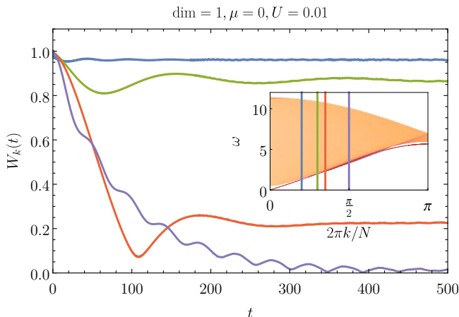
FIG. 8. Time evolution of 1-particle weight. We show, for different momenta k , the real time evolution of the 1-particle weight W_k(t) = |\langle \psi_k(0) | \psi_k(t) \rangle|^2 , where |\psi_k\rangle = \hat{V}_{1\text{ particle}}^{(k)} |\psi_g\rangle is a perturbation vector in the one particle sector of the tangent plane. The overlap in the previous equation is computed as explained in Appendix F.
