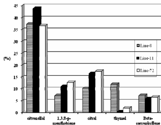
Figure 1. Comparison of major components in three essential oils (%)
