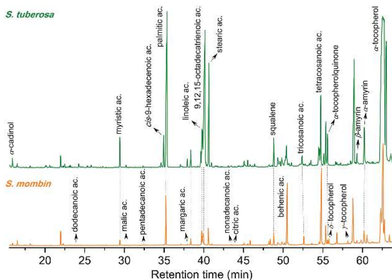
Figure 2. Chromatograms (same scale) obtained by GC-MS of the hexane extracts from Spondias leaves: green denotes S. tuberosa and oranges denotes S. mombin .
