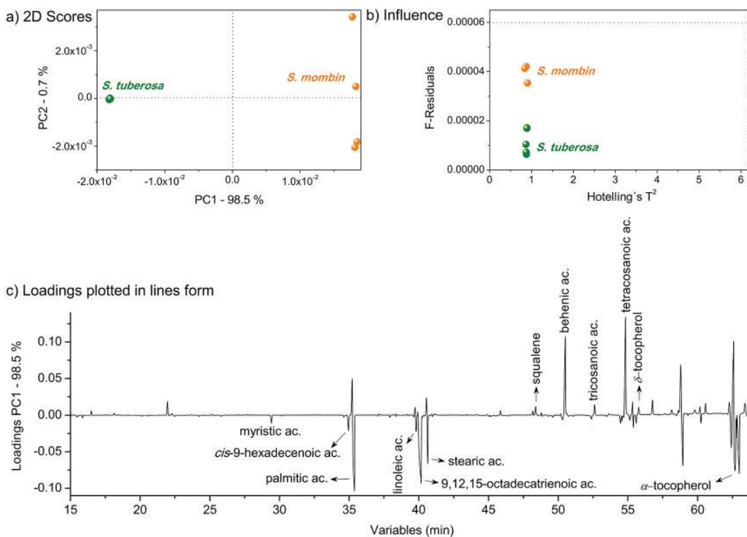
Figure 3. Chemometrics analysis: (a) bidimensional scores coordinate system (PC1 \times PC2) from S. mombin and S. tuberosa leaf extracts; (b) influence plot from Hotelling's T^2 \times F -residuals; (c) line forms of relevant loadings.
