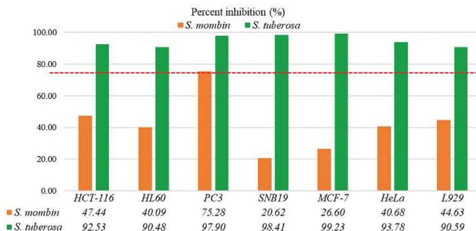
Figure 1. Inhibitory effect of hexanic extracts from leaves of S. mombin and S. tuberosa .
