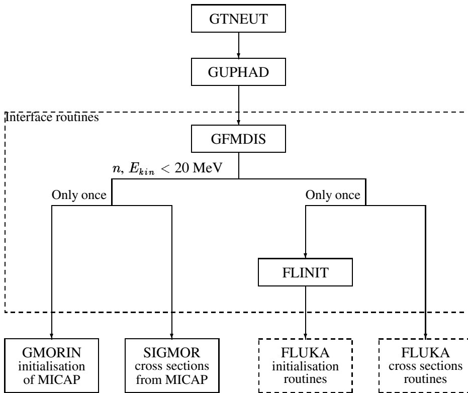
Figure 47: Program flow for calculation of the distance to the next interaction point
