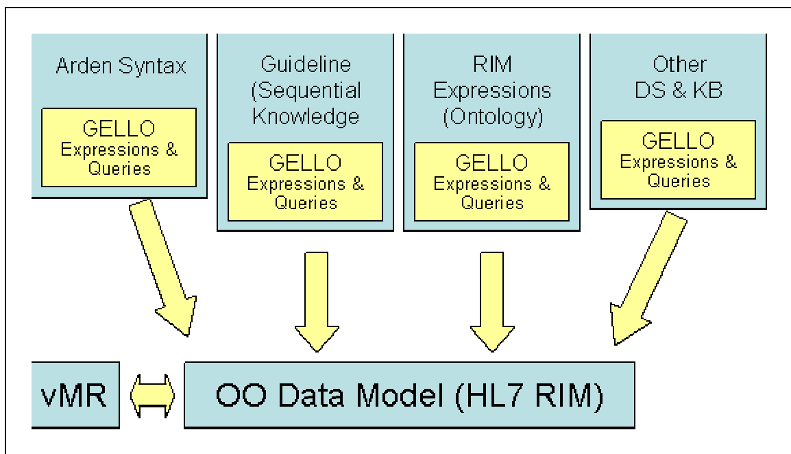
Figure 1: GELLO and its relation to Arden Syntax, GLIF, RIM and other DSs and KBs. GELLO query and expression languages can be embedded into various tools to provide the mechanisms for access and manipulation of OO data.
