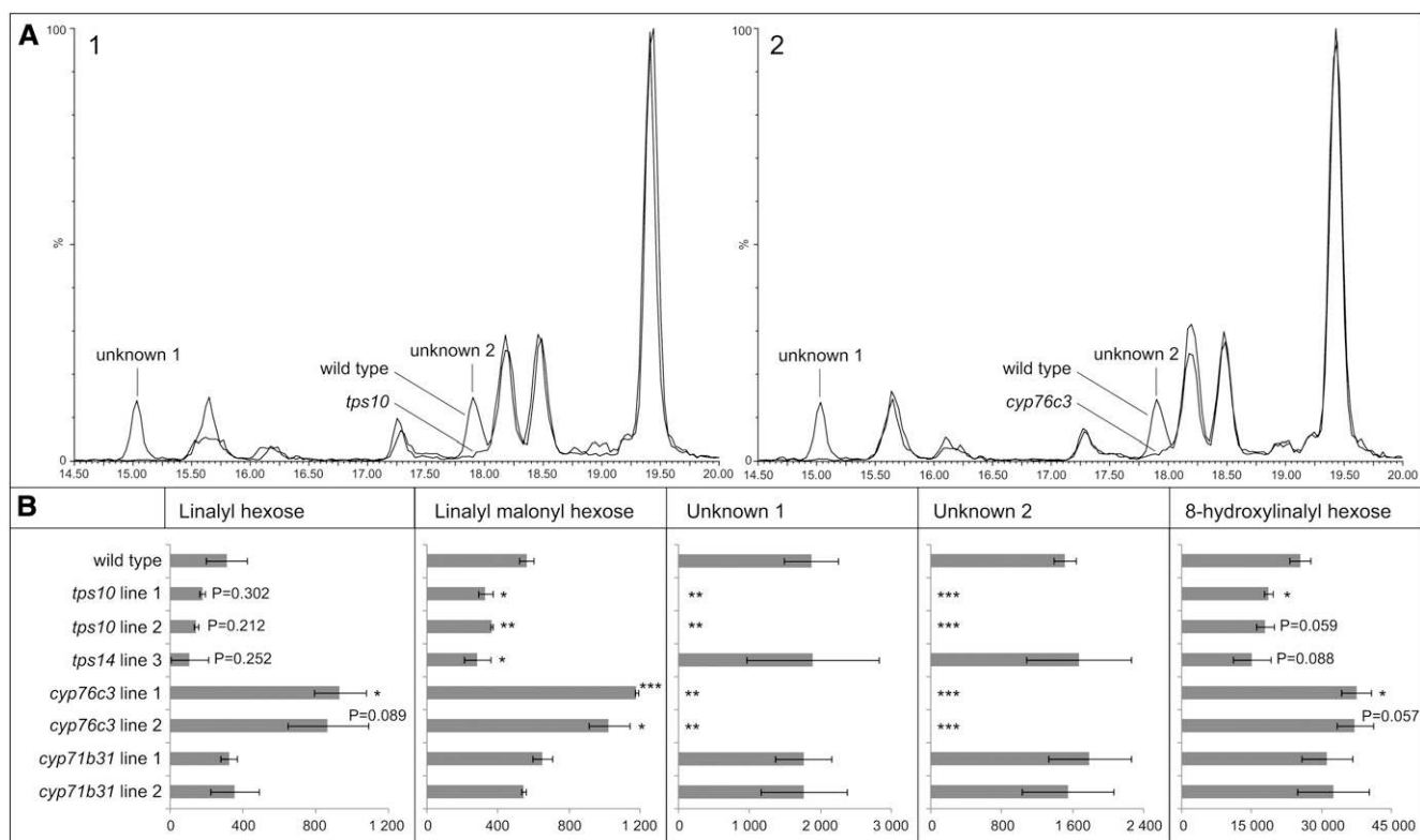
Figure 9. Targeted UPLC-MS Analysis of Linalool Derivatives in the Wild Type and TPS/P450 Insertion Mutants.
