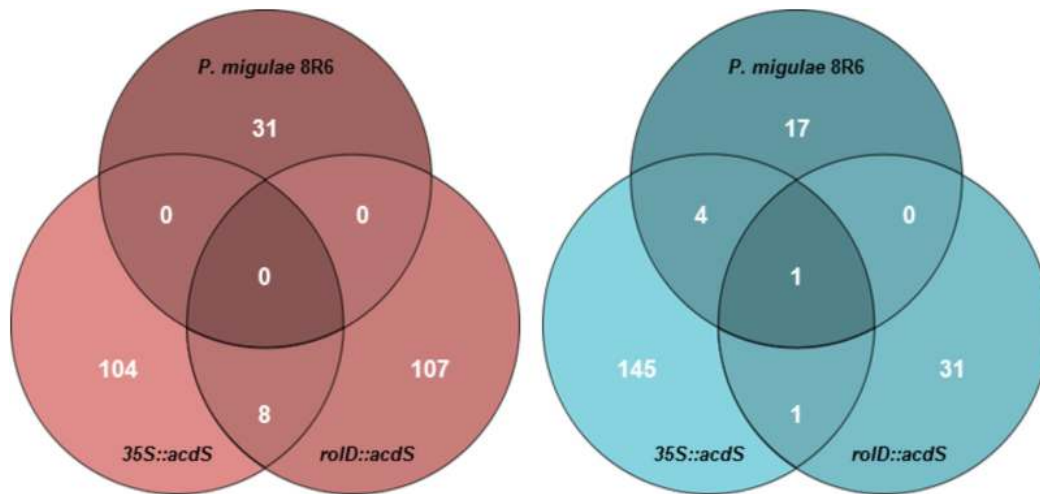
FIGURE 3 | Venn diagrams depicting the number of genes that were differentially expressed in roots of C. sativa lines expressing acdS under the control of the root-specific rolD promoter or the constitutive CaMV 35S promoter or treated with P. migulae 8R6 in the presence of salt. Up-regulated (left-hand panel) and down-regulated (right-hand panel) genes in roots 28-day-old plants treated with salt (NaCl; 15 dSm -1 ) for 3 weeks. Genes with an FDR and P -value \leq 0.05 and an absolute value of log 2 FC higher than 0.8 were considered significant.
