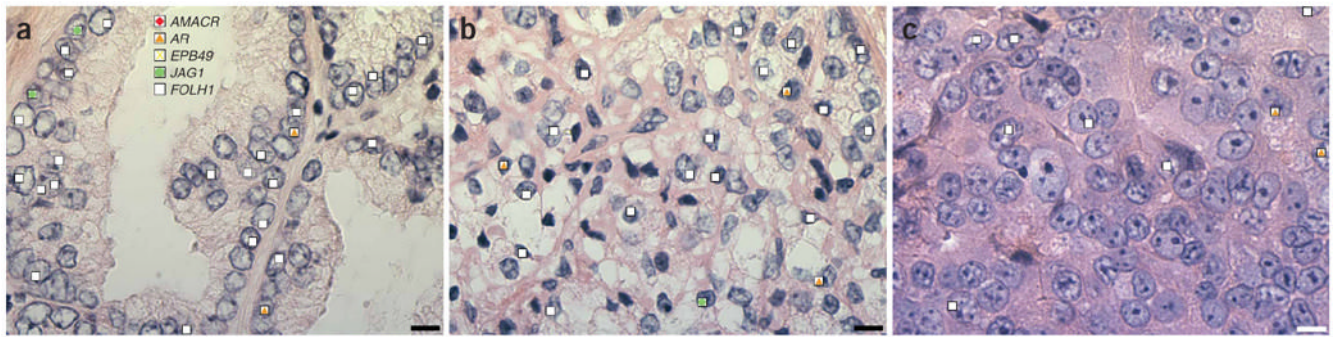
Figure 2. Correlation of single-cell multigene expression profiles with diagnostic pathology. (a–c) Hematoxylin and eosin–stained images of focal PIN (a), PCa (b) and PCaMet (c), superimposed with the gene expression data from peT-FISH analyses of three genes ( AR , JAG1 and FOLH1 ) obtained from the slide after destaining. Bars, 10 μm.
