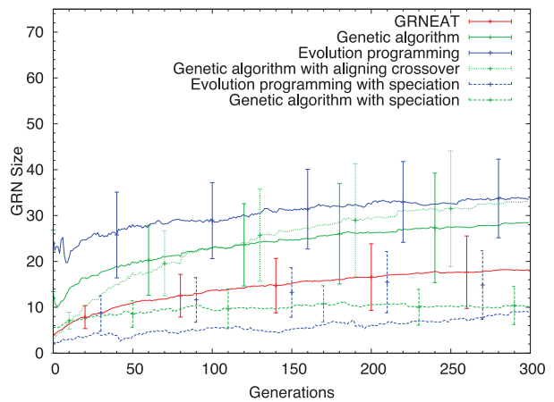
Fig. 7. Comparison of the size of the GRNs generated by GRNEAT, GA, and EP on the low-pass filter problem.
