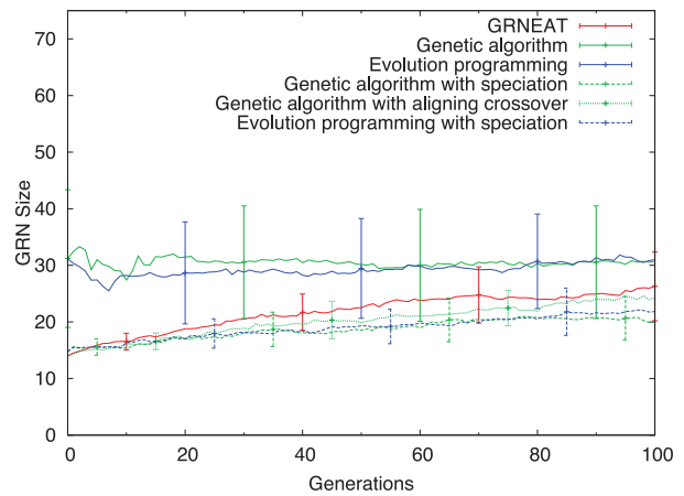
Fig. 15. Comparison of the sizes of the GRNs generated by GRNEAT, GA, and EP. The size of the GRNs generated by a GA with aligning crossover and GA, and evolution programming speciation are also plotted on this graph.
