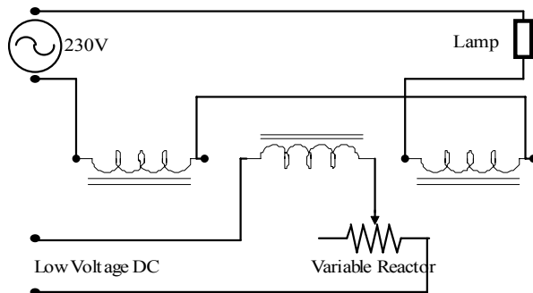
Fig. 4 Reactor Dimmer
