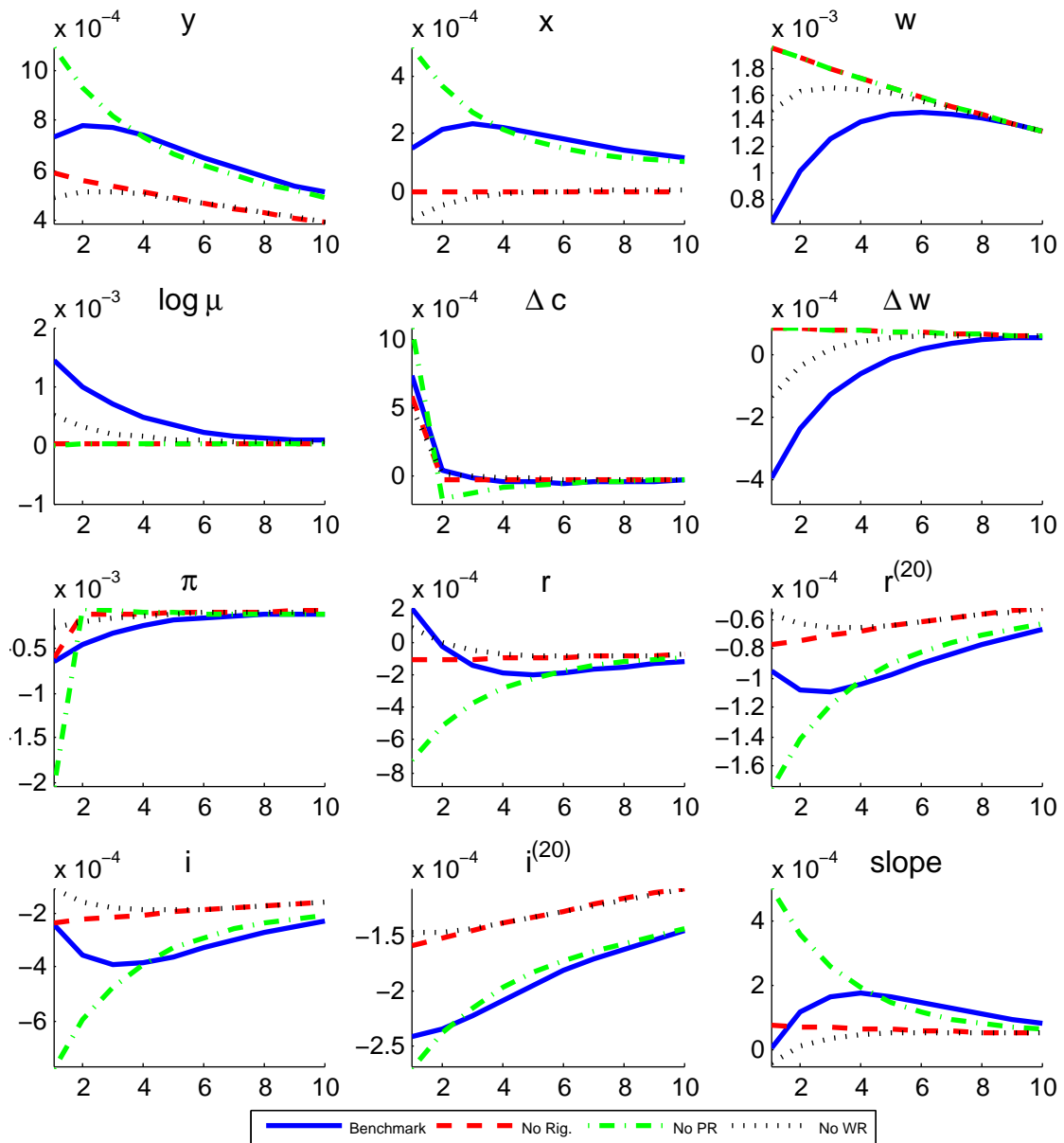
Figure B.4: Impulse responses to a one-standard deviation positive transitory productivity shock for different macroeconomic variables and interest rates. The parameter values are presented in Table B.5.
