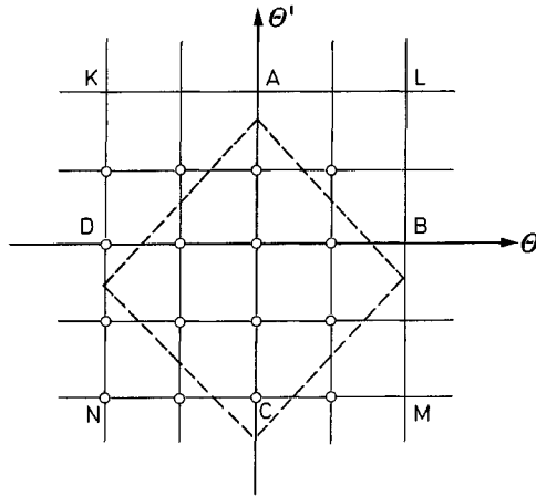
Fig. 2. Change of variables in Eq. (2.4) in the discrete case ( G = \mathbb{Z}_2 ). The final integration range consists of the points interior to the dotted square
