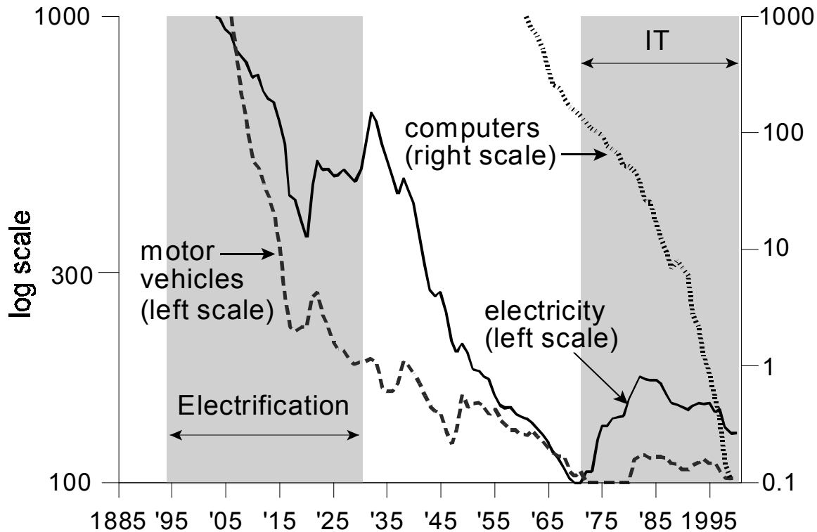
Figure 10: Price indices for products of the two GPT-eras.
