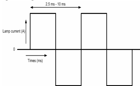
Fig 4 Current waveform of HID Lamp for stable operation
