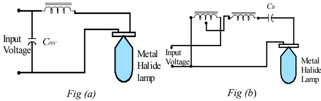
Fig. 1(a) The standard reactor circuit used in USA and Europe (b) The most popular CWA (Constant Wattage Autotransformer) circuit
