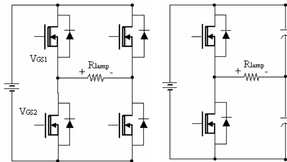
Fig. 5 (a) Full-bridge Inverter (b) Half-bridge Inverter
