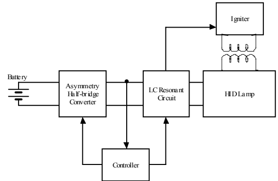
Fig. 2(b) Asymmetry Half-bridge structure of HID ballast
