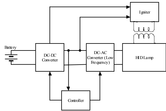
Fig. 2(a) Structure of Traditional HID Ballast
