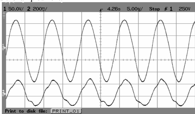
Fig 8 HID Lamp output Voltage & Current waveform
