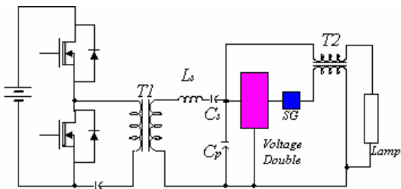
Fig.7 Asymmetry Half-bridge structure of Electronic ballast
