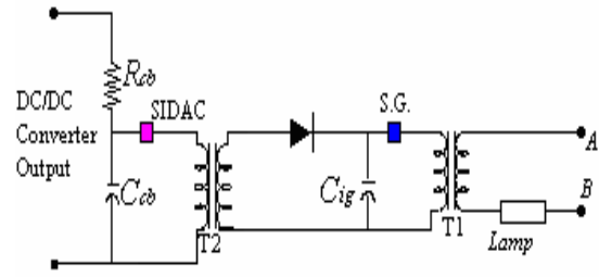
Fig 6 (a) Two-stage igniter
