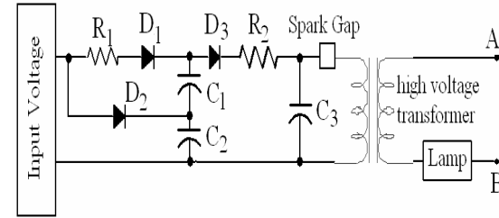
Fig 6 (b) Voltage double igniter
