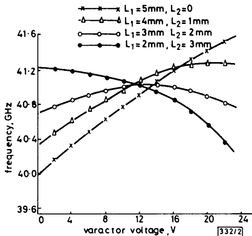
Fig. 2 Oscillator tuning characteristics
