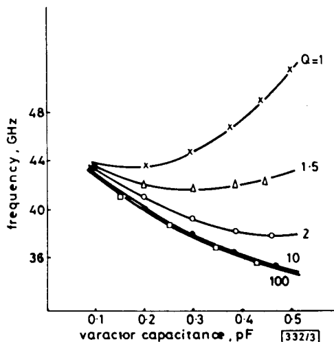
Fig. 3 Dependence of tuning characteristic on varactor Q -factor
