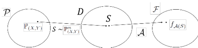
Figure 1: An illustration of differences in assumptions. Statistical learning theory analyzes the generalization behaviors of f_{\mathcal{A}(S)} over randomly-drawn unspecified datasets S \in D according to some unspecified distribution \mathbb{P}_{(X,Y)} \in \mathcal{P} . Intuitively, statistical learning theory concerns more about questions regarding a set \mathcal{P} \times D because of the unspecified nature of (\mathbb{P}_{(X,Y)}, S) , whereas certain empirical studies (e.g., Zhang et al. 2017) can focus on questions regarding each specified point (\mathbb{P}_{(X,Y)}, S) \in \mathcal{P} \times D .
