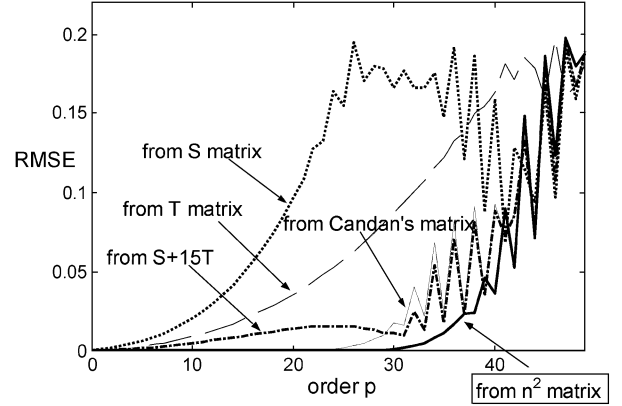
Fig. 5. Comparison of the RMSE of the DFT eigenvectors obtained from the \mathbf{S} matrix, the \mathbf{T} matrix, \mathbf{S} + 15\mathbf{T} , Candan's matrix, and the n^2 matrix where the number of points N = 50 .
