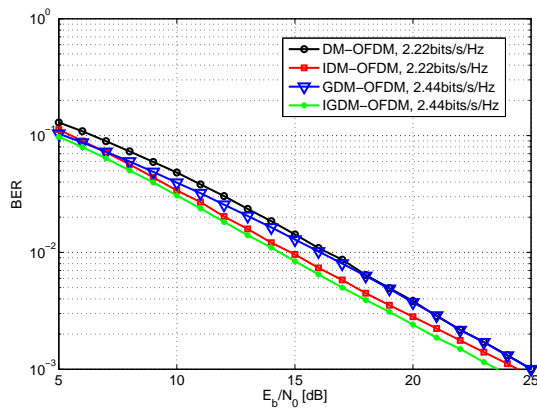
Fig. 3 Performances of GDM-OFDM and DM-OFDM with and without the interleaving technique under Rayleigh fading channel.
