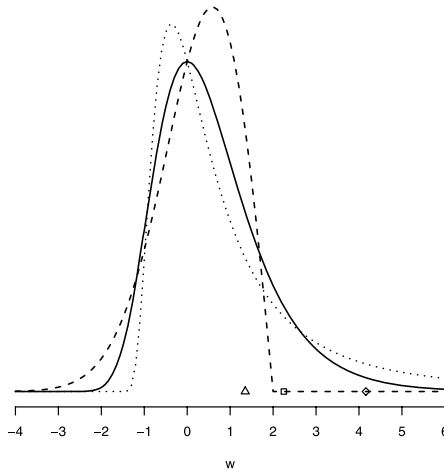
FIG. 2. Probability density function plots of Weibull distribution ( \xi = -0.5 , dashed), Gumbel distribution ( \xi = 0 , solid) and Fréchet distribution ( \xi = 0.5 , dotted). The symbols \Delta , \square and \diamond are the 90th percentile of Weibull, Gumbel and Fréchet, respectively.
