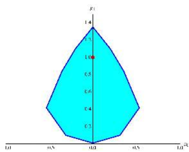
Figure 2: Outer region projections for DGP1 onto the (g_0, g_1) , (g_0, s) , and (g_1, s) planes, respectively, with 8 bins using inequalities generated with M \in \{5, 7, 9\} . The red point marks the data generating value.
