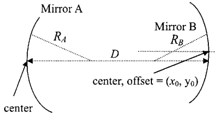
Fig. 5. Spherical-mirror-pair system.
