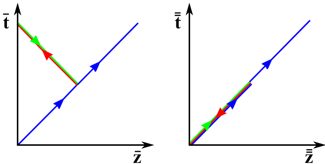
FIG. 4: Mapping of the world-line s(t) = (t, z(t)) in the original space onto the deformed spaces by means of the two different transformations. Blue lines indicate the trajectory outside of the lens (trivial mapping of all x^\mu ), the red line represents the first slab, the green line the second slab. The parametrization of the world-line in the original space is assumed to obey z(t) = t .
