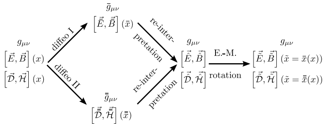
FIG. 3: Illustration and notation of the generalized “triple spacetime metamaterials” complemented by electric-magnetic rotation. The electric-magnetic rotation must act after the transformation of spacetime as these two steps do not commute.
