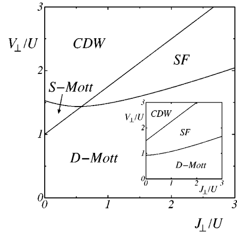
FIG. 7. Weak-coupling phase diagram of H_{\parallel}+H_{t_{\perp}}+H_{\text{int}} at t_{\perp}=t_{\parallel} and U/t=1 . This corresponds to Fig. 2. Inset shows weak-coupling phase diagram of H_{\parallel}+H_{t_{\perp}}+H_{\text{int}}+H_{\text{pair}} at t_{\perp}=t_{\parallel}=t , U/t=1 , and t_{\text{pair}}/t=0.5 . On the boundaries between the D -Mott and the S -Mott states and between the SF and the CDW states exists a massless mode C1S0. A massless mode \text{COS}\frac{1}{2} appears on the boundaries between the D -Mott and the SF states and between the S -Mott and the CDW states. The different choice of U/t does not yield qualitative changes to this phase diagram.
