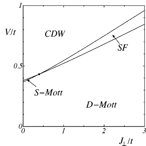
FIG. 8. Weak-coupling phase diagram of H for U/t=1 , V_{\parallel}=V_{\perp}=V , and t_{\text{pair}}=V'=0 . The tetra-critical point with C1S \frac{1}{2} is at (J_{\perp}/t, V_{\perp}/t)=(0.40, 0.43) .
