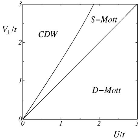
FIG. 6. Weak-coupling phase diagram of H_{\parallel}+H_{t_{\perp}}+H_{\text{int}} at t_{\perp}=t_{\parallel}=t and J_{\perp}=0 obtained from the one-loop RG equations. There is a massless mode (C1S0) on the boundary between the D -Mott and the S -Mott states while the boundary between the S -Mott and the CDW state is \text{COS}\frac{1}{2} .
